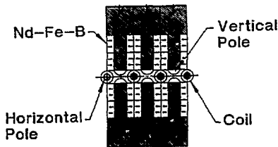
Fig. 2. EW20.0 Longitudinal View of Magnetic Structure
