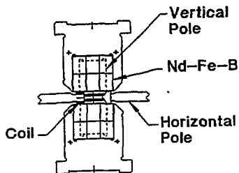
Fig. 1. EW20.0 End View of Magnetic Structure
