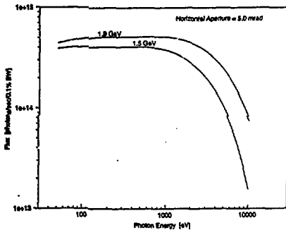
Fig. 4. Optimized M for 1.5 GeV and 1.9 GeV electron energies. Current is 0.4 A and the horizontal aperture is \pm 2.5 mrad.
