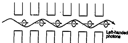
Fig. 3. Elliptical Wiggler Principle of Operation
