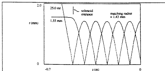
Figure 2. The orbits of ions with maximum x displacement and maximum x' divergence matched into a 2 T solenoid for a ^{132}\text{Sn}^{1+} beam with 38.7\pi mm-mr emittance at 1 keV.
