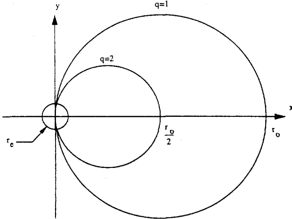
Figure 4. End view of ion and electron orbits in the solenoid.
