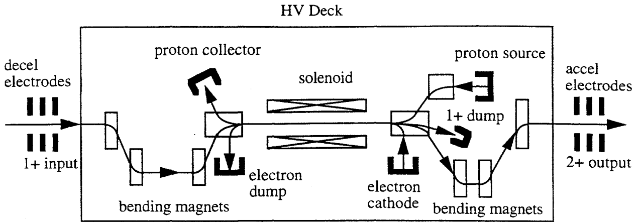
Figure 1: Electron Beam Charge State Amplifier (EBQA) single-pass configuration
