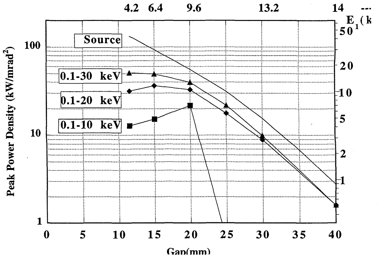
Fig. 2 Calculated peak power densities for the entire Undulator A spectrum as a function of undulator gap and for the three energy bands indicated. The first harmonic energy corresponding to the undulator gap is shown at the top.
