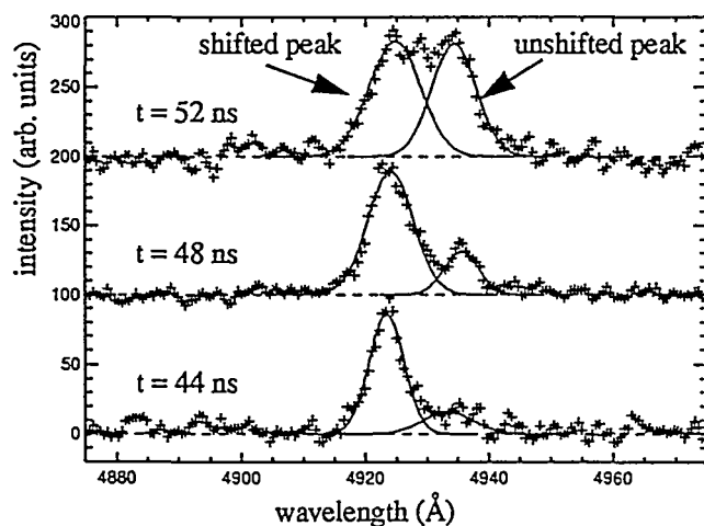
FIGURE 8. A temporal sequence of lineouts for the Ba II 6s\ ^2S_{1/2}-6p\ ^2P_{1/2} transition, measured adjacent to the PBFA II anode. Each successive time step is displaced by 100 intensity units to facilitate viewing. Gaussian fits to the peaks (solid curves) obtained with the ROBFIT code are superimposed on the data (plus signs). The unshifted (zero field) wavelength is 4934.1 Å.
