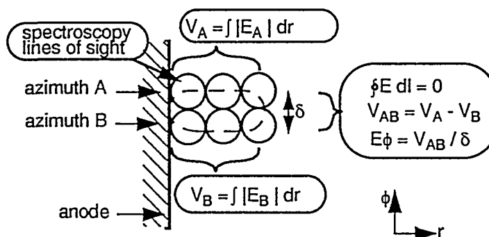
FIGURE 6. Top view of the diode AK gap illustrating the method used to determine the non-radial electric fields from the Stark shift measurements. The circles represent individual spectroscopic lines of sight that are approximately 2 mm in diameter. The dashed curve illustrates the path for the line integral. In actual experiments a larger array of points (up to eighteen total) is used to obtain more complete measurements of the radial and azimuthal dependence.
