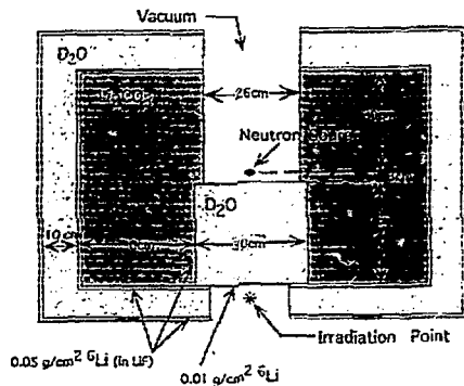
Assembly Design #4 (Blue et. al.)
