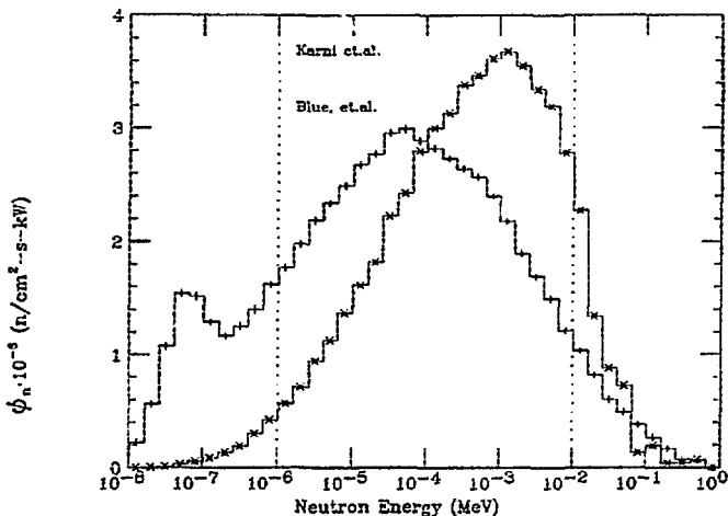
Figure 13: Neutron spectral shape for assembly designs #1 (BeO moderator by Blue) and #3 ( {}^7\text{Li}/\text{Pb} by Karni). The \Phi_{u/P} in both cases is about equal to 4.7 \times 10^7 (n/cm 2 -s-kW). Both spectrums are produced from incident 2.5 MeV proton beams.
