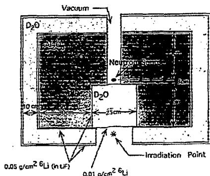
Assembly Design #2 (Blue et. al.)
