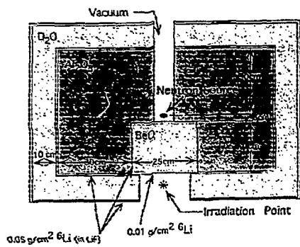
Assembly Design #1 (Blue et. al.)
