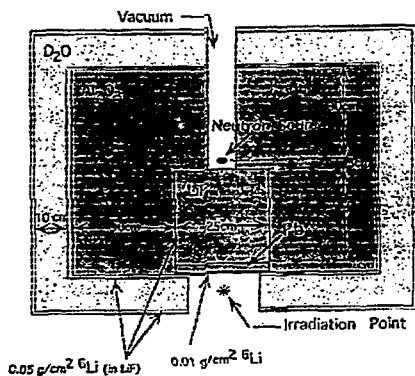
Assembly Design #3 (Greenspan)
