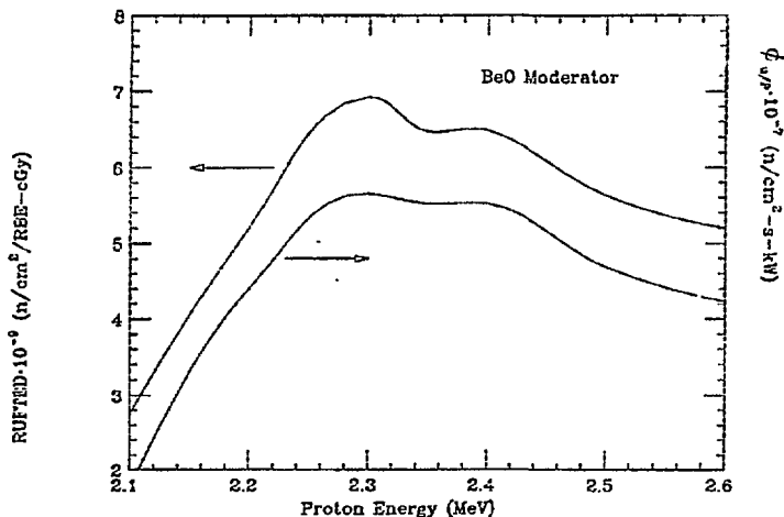
Figure 9: RUFTEd & \Phi_{u/P} vs. proton energy and BeO moderator (Assembly design #1) for various proton energies. For RUFTEd values the \Phi_{u/P} was held constant at 4.69 \times 10^7 (n/cm 2 -s-kW). For \Phi_{u/P} values the RUFTEd was held constant at 5.63 \times 10^9 (n/cm 2 /RBE-cGy).
