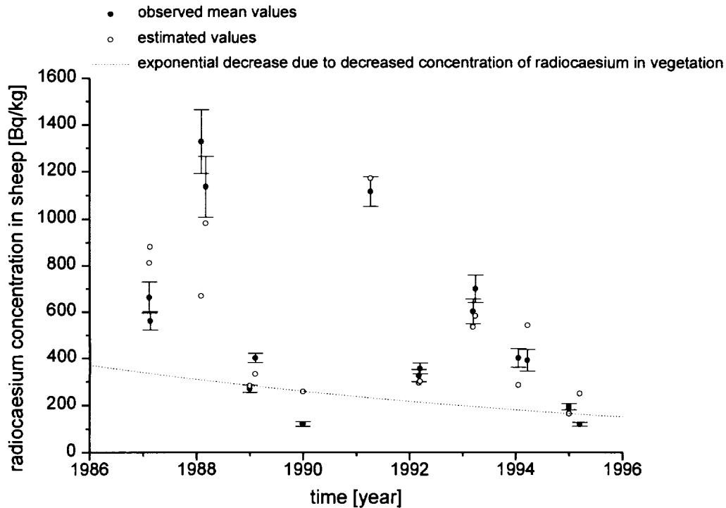
Figure 7.2: Estimated values for 137 Cs concentration in sheep are compared with the mean of the observations for each year \pm std. error of mean. The dot-and-dash line illustrates the underlying exponential decrease in 137 Cs concentration in sheep due to decrease in contamination level in vegetation. Time for appearance of fruit bodies is set to 15.08, and the relative importance between the different levels of fungi abundance is 1:4:9.
