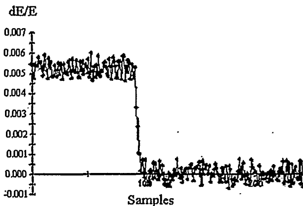
Fig. 3 Injector Energy lock- Effect of closing the loop ( E = 45 \text{ MeV} )
