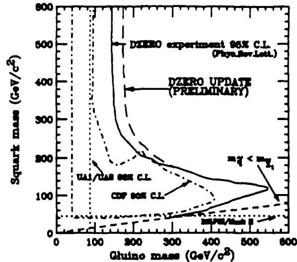
FIG. 3. The squark and gluino mass limits are presented in this plot. The long dashed line marks the preliminary DØ 95% confidence level excluded region from the combination of the three jet and four jet analyses. The solid line indicates the DØ three jet search PRL (2) result. The region below the dashed line labeled m_q < m_g , is excluded since there the squark becomes lighter than the LSP. Other published limits from CDF, UA1, UA2, and DELPHI (9) are displayed as well.
