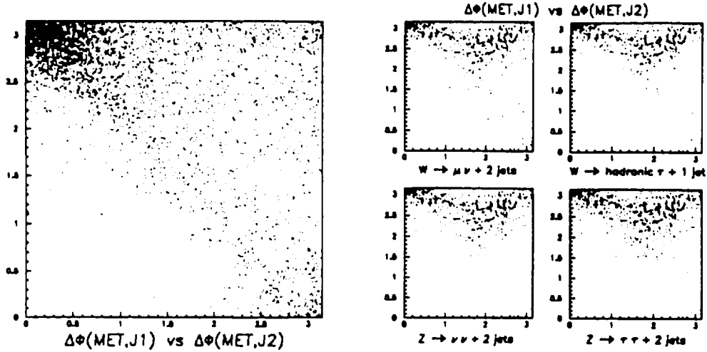
FIG. 1. On each plot the opening angle between the \cancel{E}_T vector and the leading jet runs up the vertical axis, and the angle between \cancel{E}_T and the next leading jet runs along the horizontal axis. On the left is shown events from a low E_T threshold single jet trigger with an offline \cancel{E}_T > 15 GeV cut applied. Monte Carlo of some vector boson backgrounds are displayed at right.
