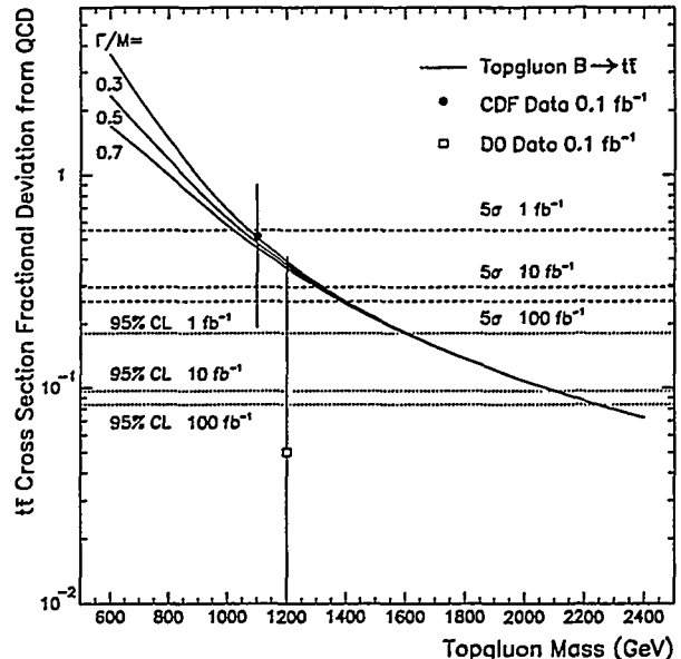
Figure 3: The fractional difference between the t\bar{t} cross section and the QCD prediction is shown for topgluons (solid curves), CDF data (solid circle), and D0 data (open box). The projected 5\sigma uncertainty (dashed lines) and 95% CL (dotted lines) on the measured t\bar{t} cross section can be compared with the topgluon prediction to determine the discovery reach and exclusion reach of the Tevatron at the luminosities of 1, 10 and 100 \text{ fb}^{-1} .
