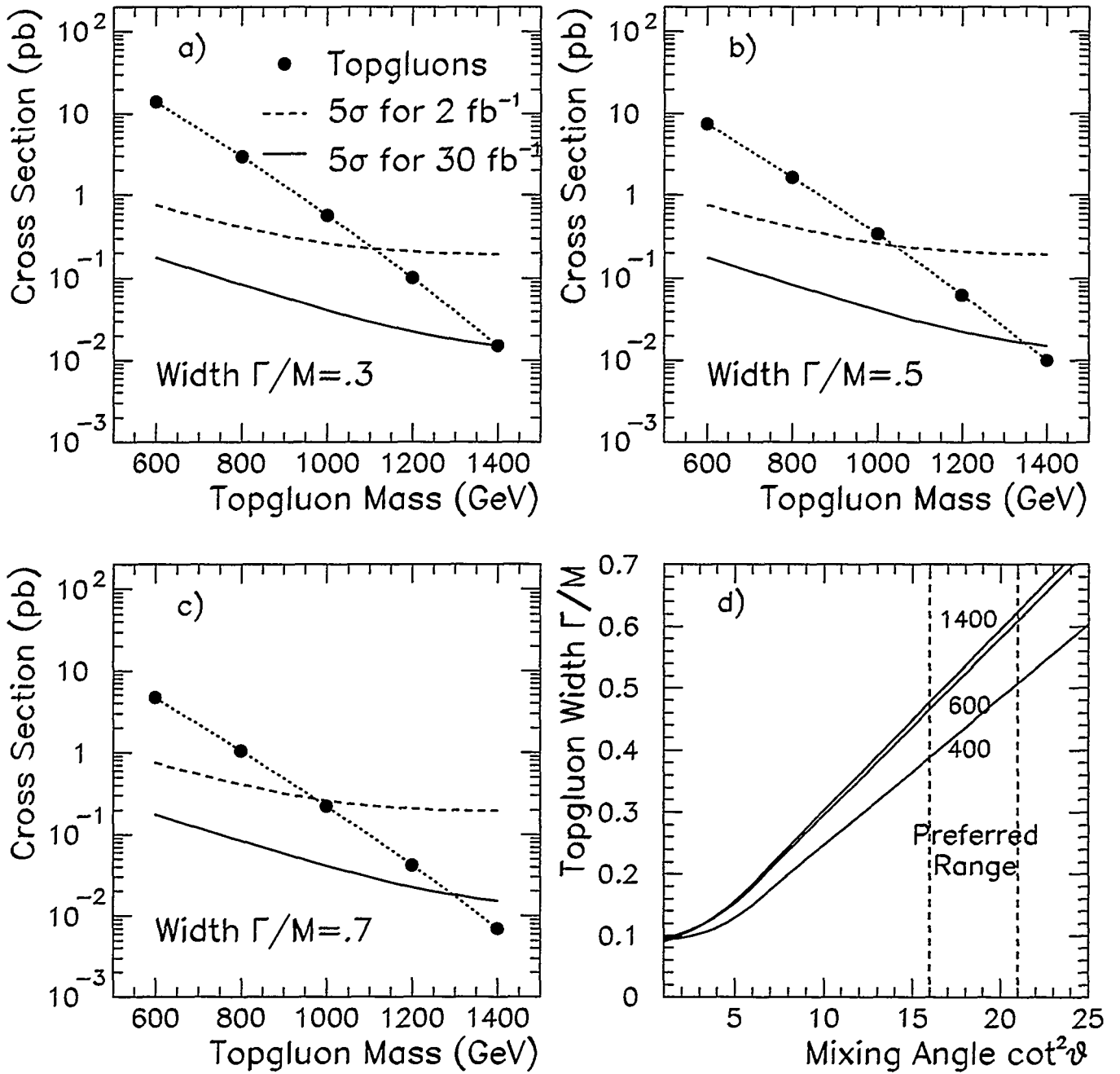
Figure 2: The mass reach for t\bar{t} decays of topgluons of width a) 0.3 M, b) 0.5 M, and c) 0.7 M. The predicted cross section for topgluons (points) is compared to the 5\sigma discovery reach of the Tevatron with a luminosity of 2 \text{ fb}^{-1} (dashed) and 30 \text{ fb}^{-1} (solid). All cross sections are for t\bar{t} with invariant mass within 25% of the topgluon peak. In d) the solid curves relate topgluon width and the mixing angle, \theta , between SU(3)_1 and SU(3)_2 for 3 different topgluon masses. The vertical dashed lines indicate the theoretically preferred range of mixing angle [6].
