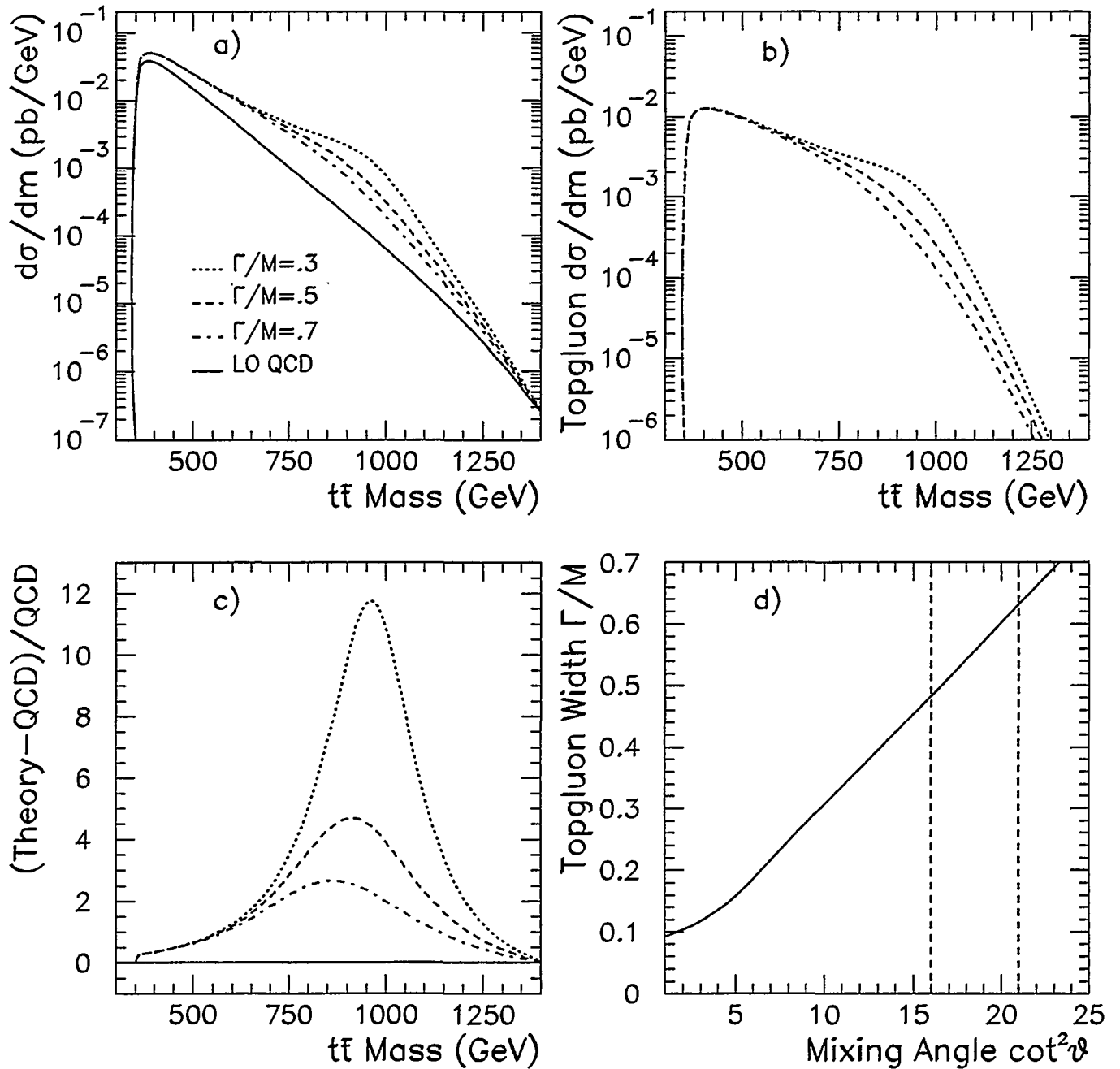
Figure 1: Lowest order parton level predictions for a 1000 GeV topgluon decaying to t\bar{t} displayed as a function of t\bar{t} mass. a) The cross section for the LO t\bar{t} background from QCD (solid) is compared to the coherent sum of LO QCD and a topgluon of fractional width \Gamma/M = 0.3 (dots), 0.5 (dashes) and 0.7 (dotdash). In b) the QCD prediction has been subtracted leaving only the topgluon signal and the interference between QCD and topgluons (constructive beneath peak, destructive above peak). c) The fractional deviation above the QCD prediction produced by the presence of a topgluon. d) The solid curve relates the topgluon width and the mixing angle, \theta , between SU(3)_1 and SU(3)_2 for a 1000 GeV topgluon. The vertical dashed lines indicate the theoretically preferred range of mixing angle [6].
