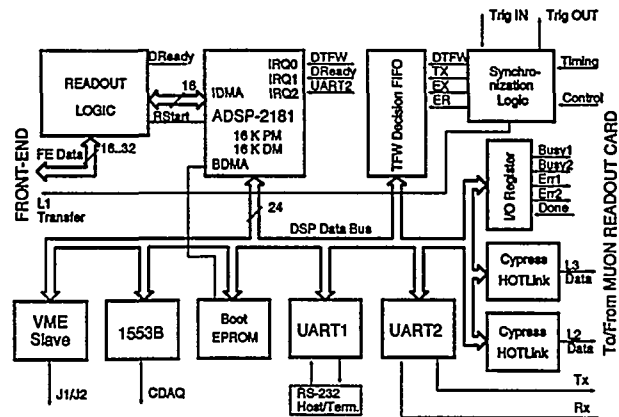
Figure 4: Muon Readout Controller. DTFW - L1 Accept + L2 Accept + L2 Reject, TX - TFW crossing number, EX - Event crossing number, ER - Event turn number.
