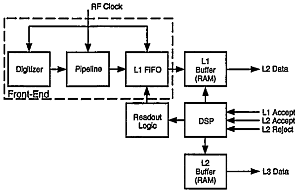
Figure 3: Muon system buffering scheme. DSP - digital signal processor.
