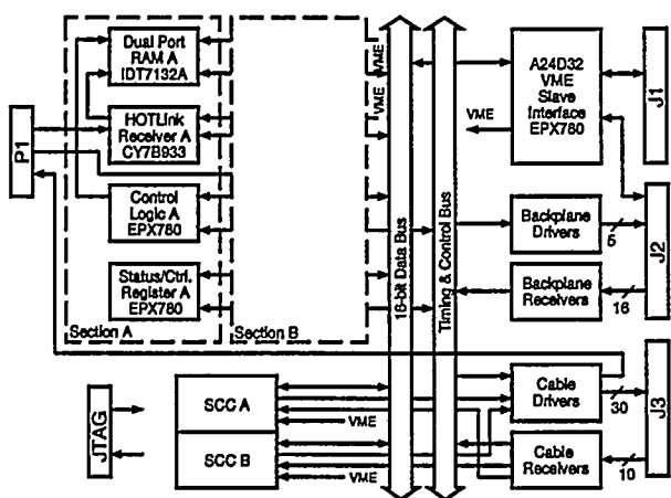
Figure 5: Muon Readout Card. VME - VME command.
