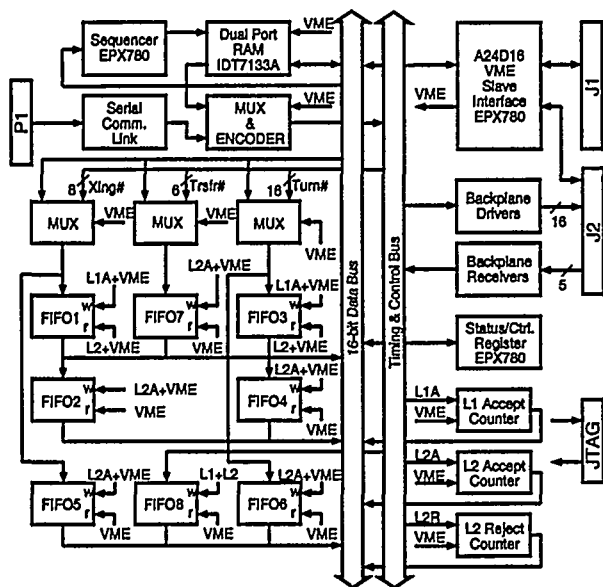
Figure 6: Muon Fanout Card. L1A - L1 accept, L2A - L2 accept, L2R - L2 reject, L2 - L2A + L2R, VME - VME command.
