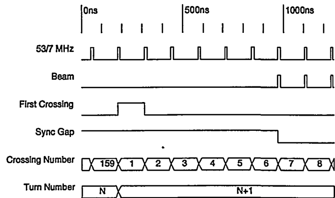
Figure 2: Timing diagram showing relevant signals at first crossing
