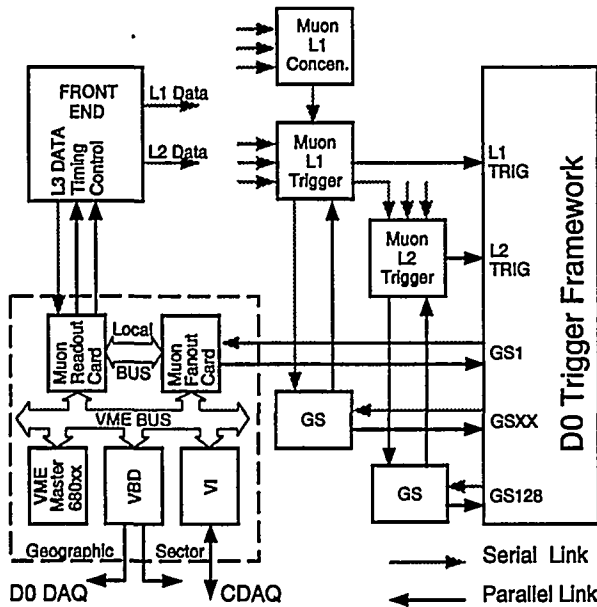
Figure 1: D0 muon trigger architecture. GS - geographic sector, SL - Serial Link.
