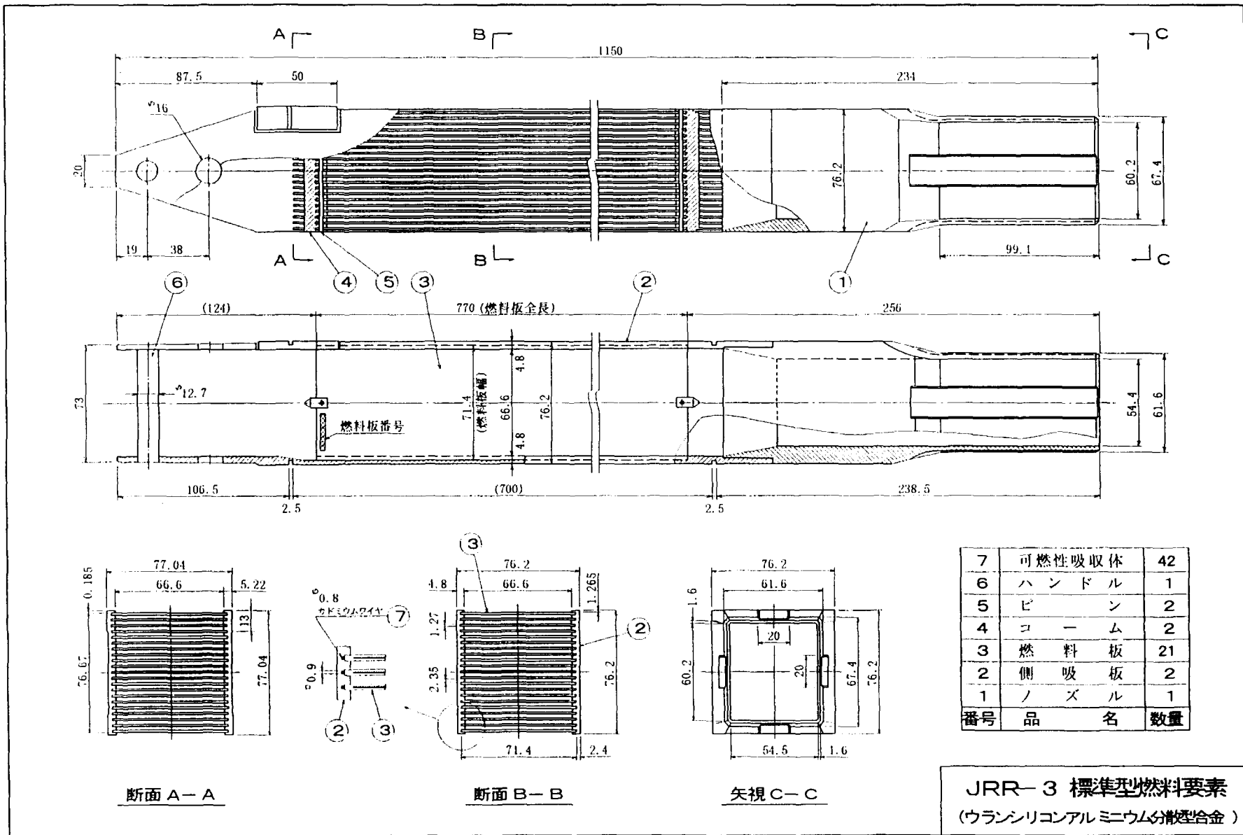
Fig 1.1.1 JRR-3 standard type fuel element (Silicide fuel)
