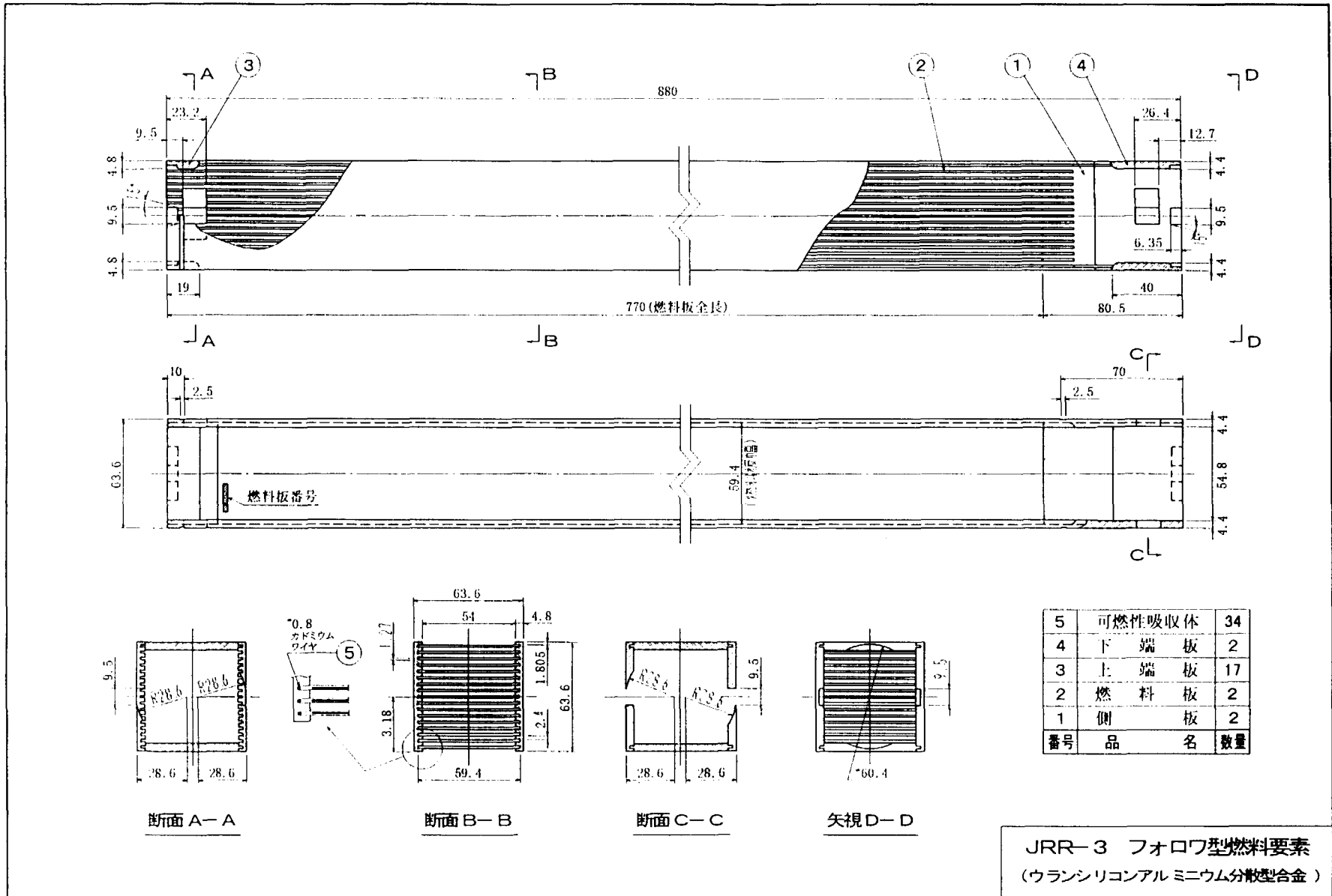
Fig.1.1.2 JRR-3 follower type fuel element (Silicide fuel)
