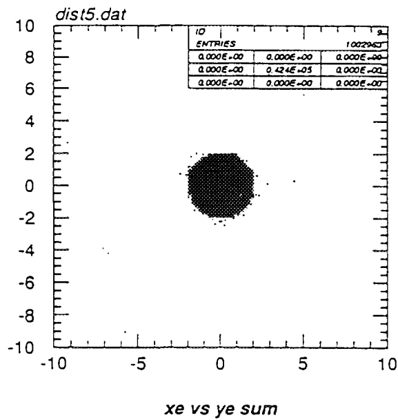
Fig.8 The beam profiles behind the collimator system
