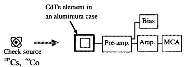
Fig.7 Block diagram of the experiment.
