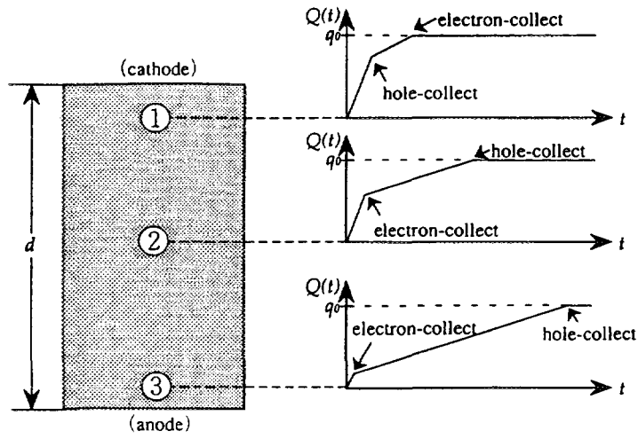
Fig.1 Pulse shape in relation to the interaction position (planar type detector).
