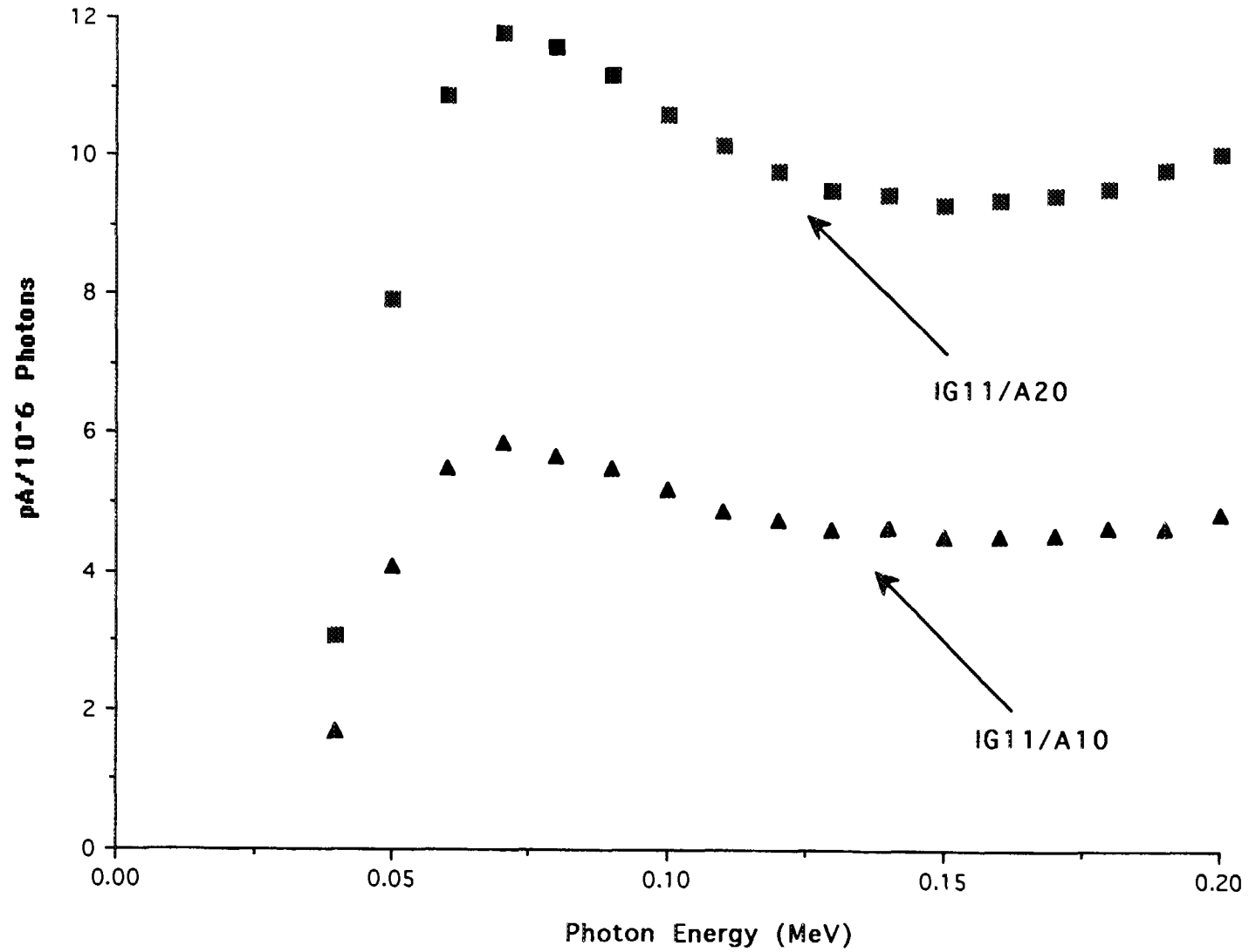
Fig.6 Response function of ionization chambers in the lower energy region (filled with 1 MPa or 2 MPa argon)
