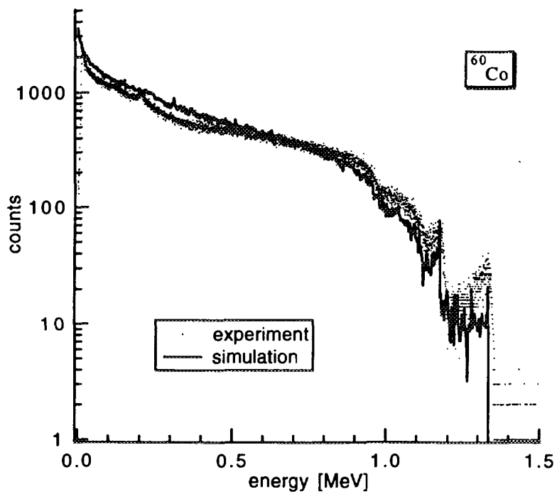
Fig.8-2 Results of the simulation compared with the results of the experiment ( ^{60}\text{Co} ).
