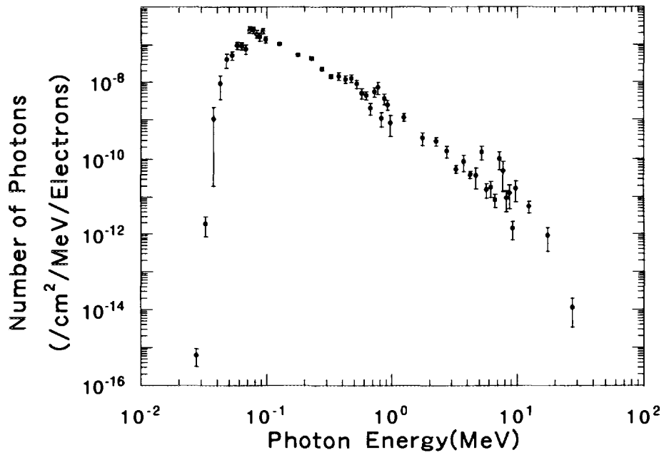
Fig. 4 Photon Energy Distribution at the Air-Duct
