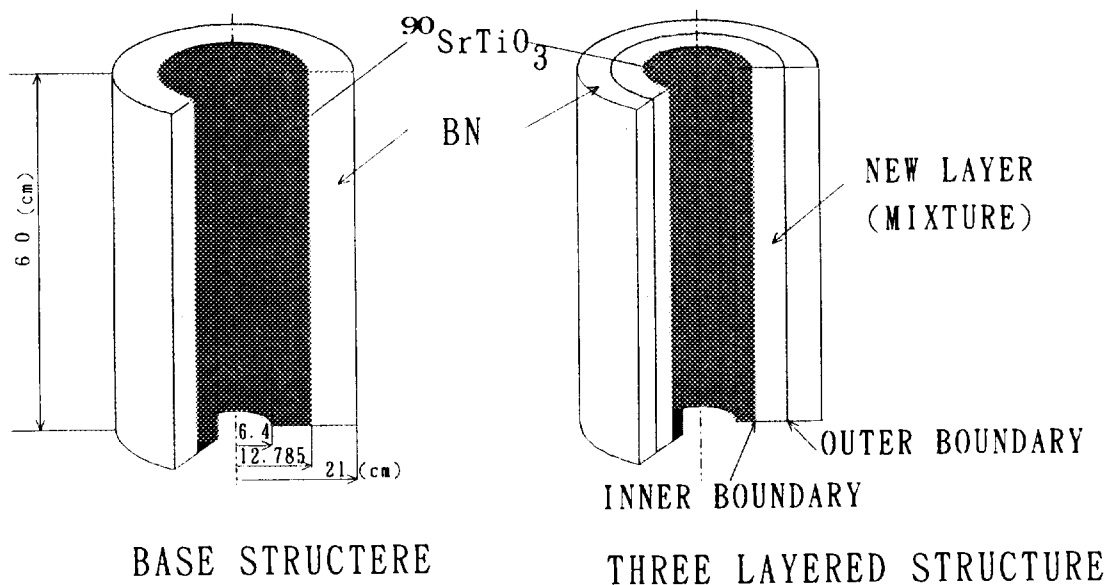
Figure 1. Calculation model.
