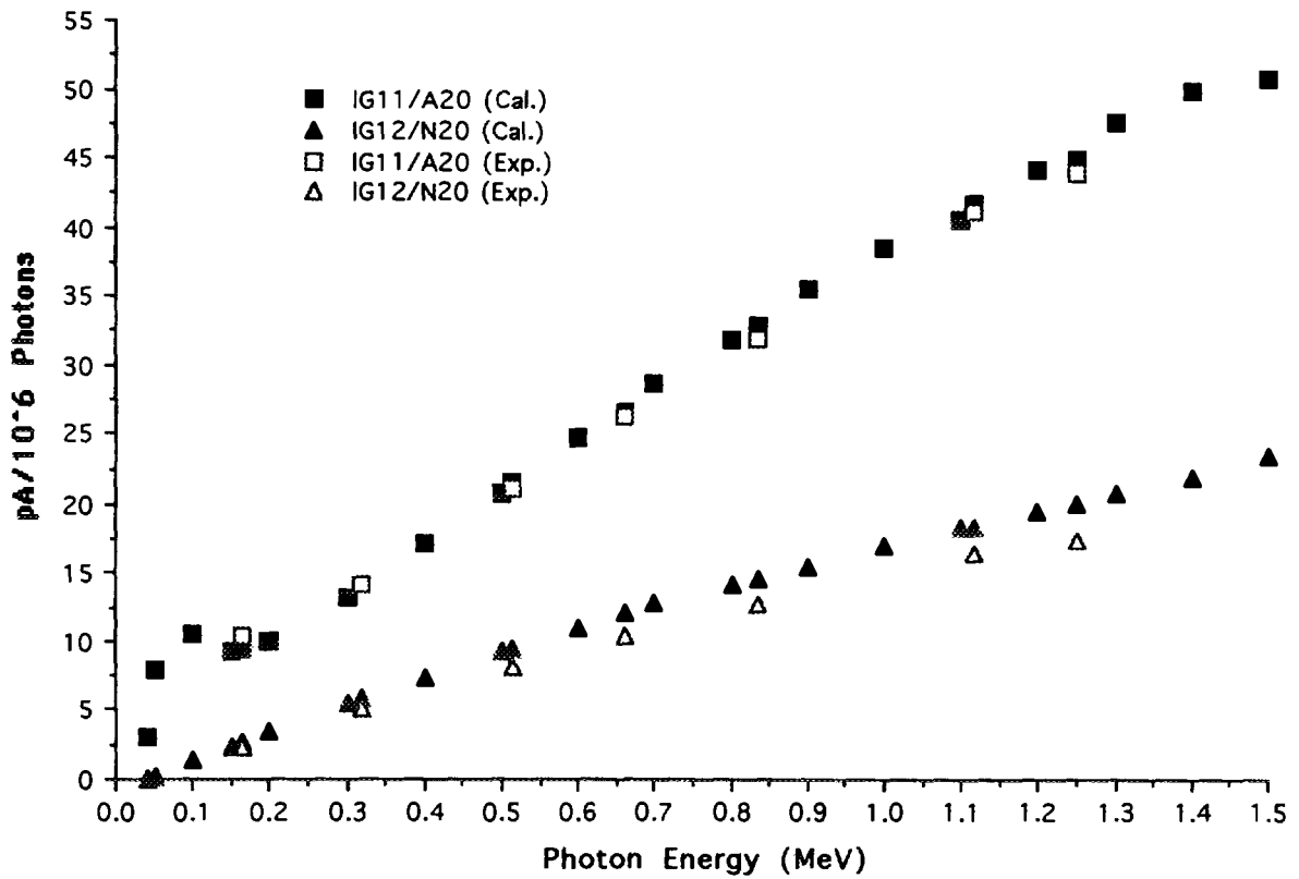
Fig.5 Response function of ionization chambers (filled with 2 MPa argon or nitrogen)
