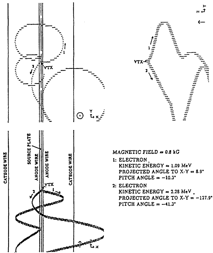
Fig. 6. An example of the simulated 0\nu\beta\beta event emitted back to back at DCBA [9].
