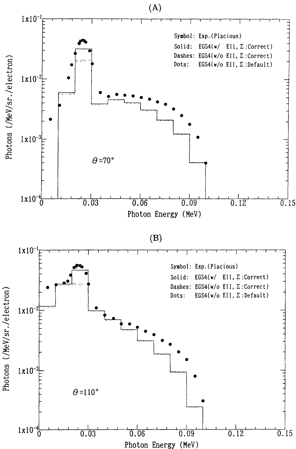
Figure 1: Spectra of the bremsstrahlung and K-X rays from a Sn target ( 21.6 \text{ mg/cm}^2 ). A 100 keV electron beam is normally incident on the target. Photons emitted toward (A) 70^\circ and (B) 110^\circ from the incident electron direction are shown, respectively. The closed circle is a measurement by Placious. The solid and dashes line show the EGS4 calculation with and without electron-impact ionization (Møller scattering and bremsstrahlung underestimation is corrected). The dotted line shows the EGS4 calculation in the condition that electron-impact ionization is not included and the Møller scattering and bremsstrahlung underestimation is not corrected. The dashed line and solid lines overlap many times.
