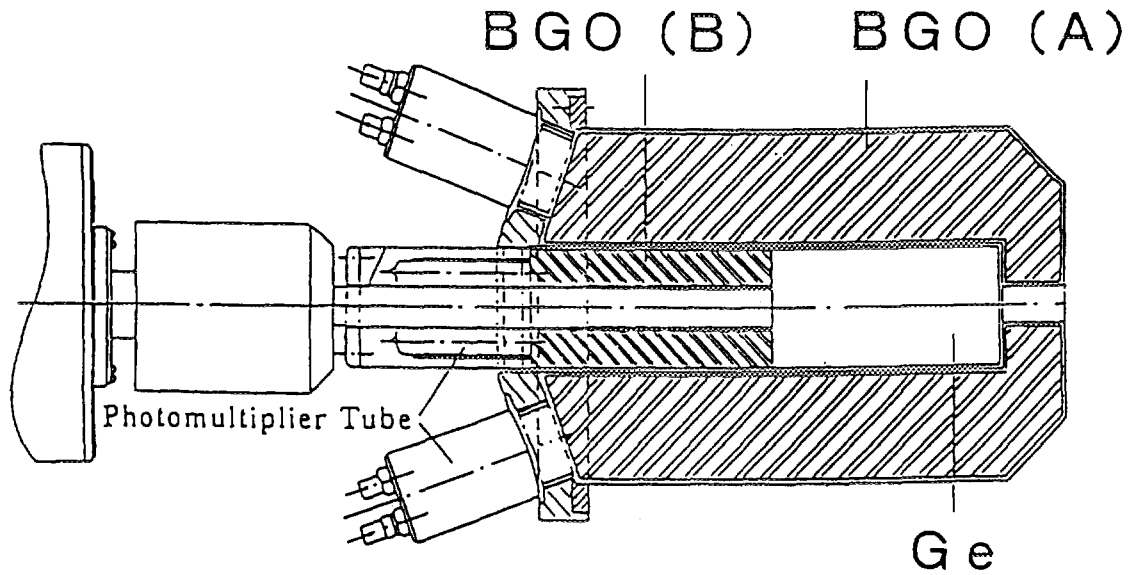
Fig.1 Cross-Sectional View of Detector of Compton Suppression System
