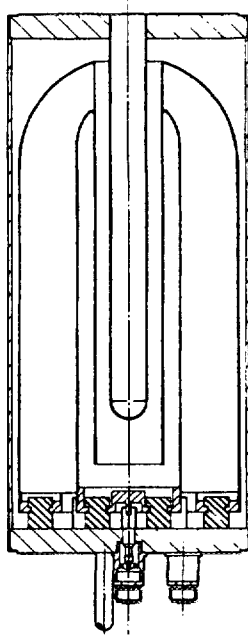
Fig.1 Sectional view of a one-inch-diameter reentrant-well IG=11 pressure ionization chamber
