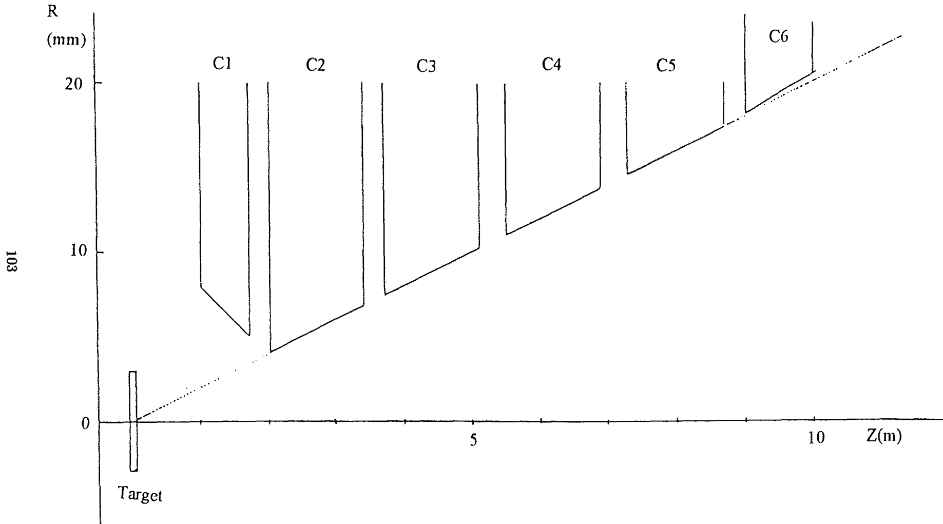
Fig.2 The schematic drawing of the holes of the collimator system together with the neutral beam production target
