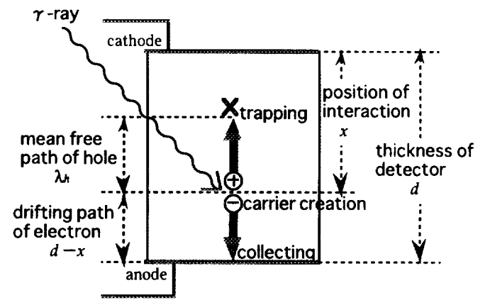
Fig.5 Hole trapping phenomena in the CdTe detector.
