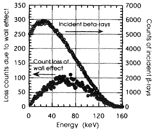
Fig.8 Count loss by wall effect calculated with ^{14}\text{C} sample gas and \text{CH}_4 counting gas at 0.5 \times 10^5 \text{ Pa} when \text{AE}=511.2\text{keV} and \text{AP}=0.2\text{keV}
