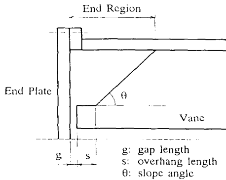
Fig. 5 Cross section of the RFQ end region
