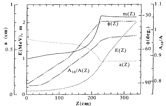
Fig. 1 RFQ parameters as a function of distance along the beam line in the RFQ
