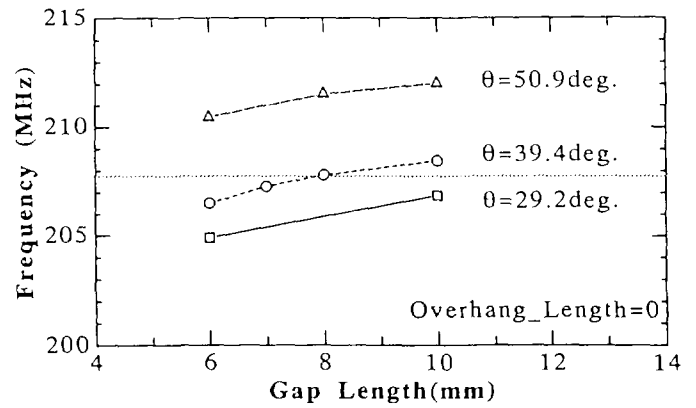
Fig. 6 Resonance frequency as a function of gap length for vane slope angle of 29.2, 39.4 and 50.9 deg. calculated with MAFIA
