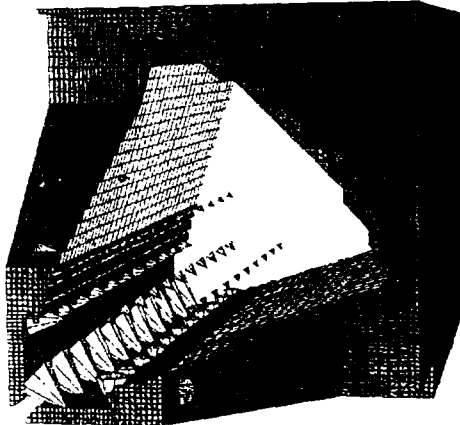
Fig. 4 Three-dimensional RFQ structure with vane end region generated with MAFIA. Arrow shows the electric field vector.
