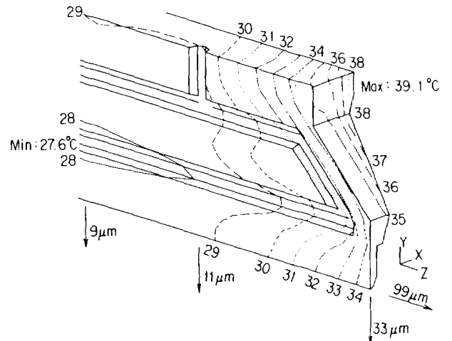
Fig. 8 Temperature distribution and displacement of the RFQ vane
