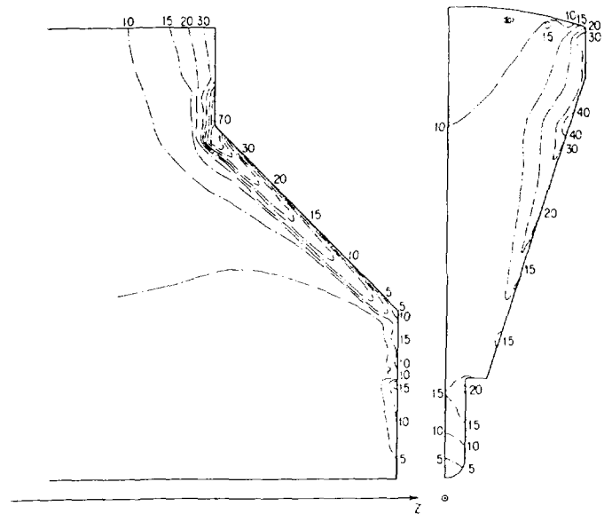
Fig. 7 RF peak power loss density in W/cm^2 along the surface of the vane. (60%Q is assumed.)
