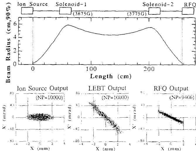
Fig. 2 Beam envelope in the LEBT, and x-x' emittance diagrams at the output positions of the ion source, LEBT and RFQ
