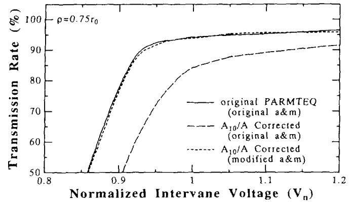
Fig. 3 Transmission rate of the RFQ as a function of normalized intervane voltage, V_n . ( 1V_n=113kV )
