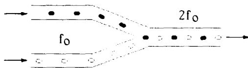
Fig. 1. Principle of a two channel funneling line.
