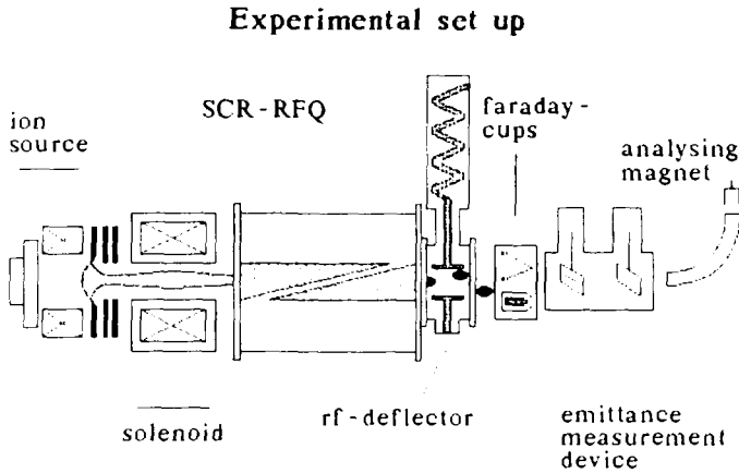
Fig. 3. The experimental set up of the defunnel line.
