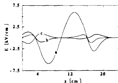
Fig. 2. The deflecting field component E_x(x,z) (a), the corresponding longitudinal field component E_z(x,z) (b), and E_z for a particle in the center of an adjacent bunch (c).
