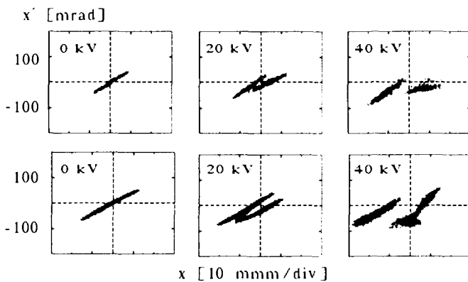
Fig. 6. The x, x' -emittance as a function of the deflector voltage. The results of the simulations are shown on the top, those of the experiments on the bottom ( I=1.2 mA).
