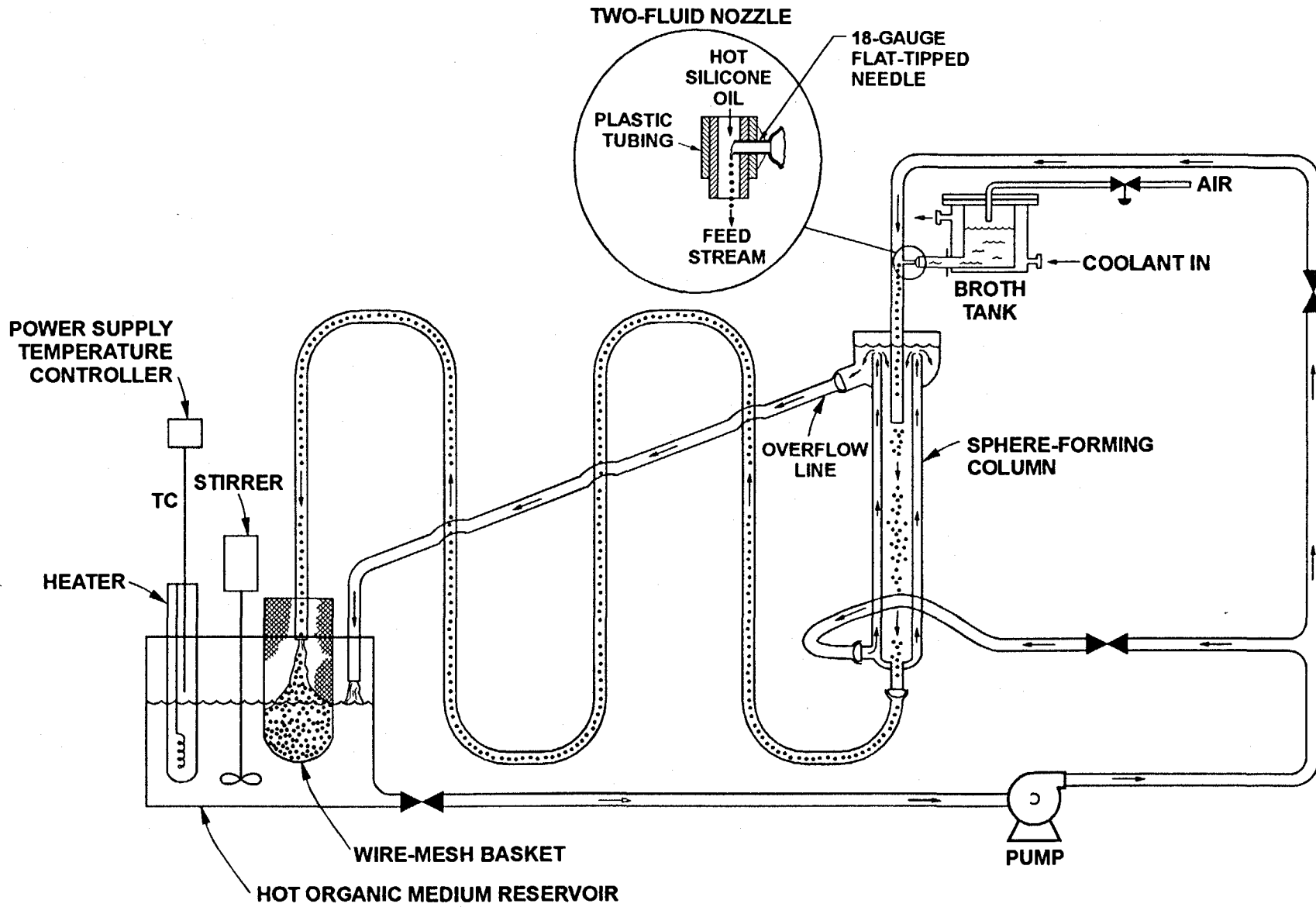
Fig. 1. Schematic of HMTA internal gelation process experimental apparatus
