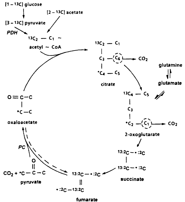
FIG. 2. Label distribution in TCA cycle intermediates from [1- 13 C]glucose and [2- 13 C]acetate. [1- 13 C]-Glucose yields [3- 13 C]pyruvate, which may yield [2- 13 C]acetyl-CoA through pyruvate dehydrogenase (PDH) or, in glia, [3- 13 C]oxaloacetate through pyruvate carboxylase (PC). In the first case 2-oxoglutarate (and hence glutamate and glutamine) is labeled in the C-4 position ( 13 C); in the latter case the label appears in the C-2 ( 13 C). In glia [2- 13 C]acetate yields [2- 13 C]acetyl-CoA, which labels 2-oxoglutarate in the C-4. In the symmetrical succinate step the label is scrambled (symbolically 13:2 C or 2:13 C). The possible scrambling of label ( 13 C) due to equilibration of oxaloacetate with fumarate is indicated by the broken arrow.
