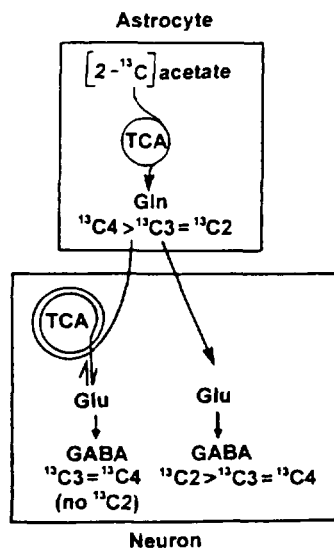
FIG. 3. Formation of GABA from [2- 13 C]acetate. In glia [2- 13 C]-acetate is converted to 13 C-labeled glutamine (Gln), which is transferred to GABAergic neurons. Here the Gln may be converted directly to GABA via glutamate (Glu), yielding GABA with a labeling of the C-2, C-3, and C-4 positions identical to the labeling of the C-4, C-3, and C-2 of Gln, respectively. Some of the Gln, however, is metabolized through the neuronal TCA cycle before being converted to Glu and GABA, leading to scrambling of the label in the C-4 of Gln between the C-3 and C-4 in GABA due to the symmetry of succinate (see Fig. 1).
