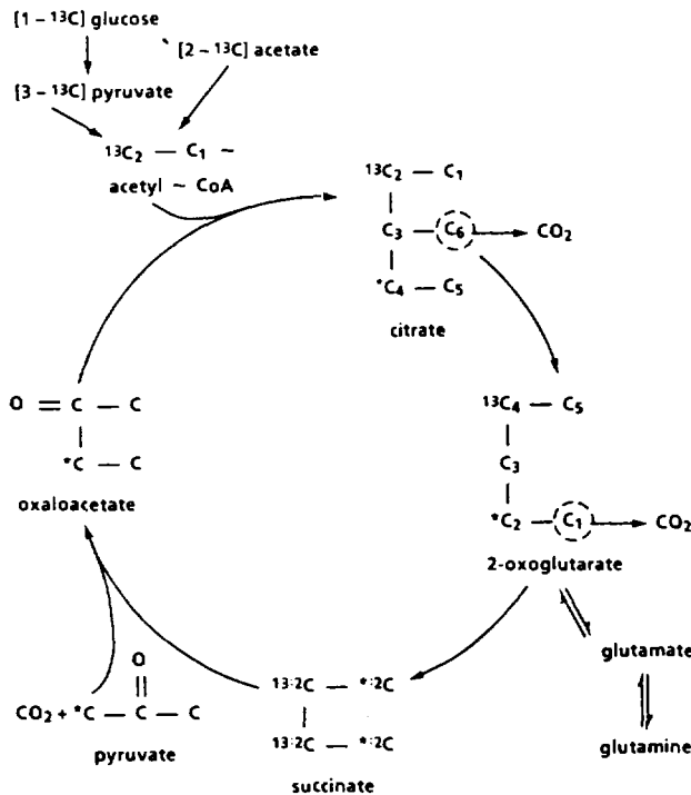
FIG. 1. A simplified scheme of the TCA cycle shows the conversion of [1- 13 C]glucose and [2- 13 C]acetate to [2- 13 C]acetyl-CoA and hence the labeling of the C-2 position in citrate and the C-4 position in 2-oxoglutarate. Because succinate is symmetrical, the label is distributed equally between the C-2 and the C-3 positions (symbolically 13 C 2 ) before formation of oxaloacetate. [1- 13 C]-Glucose yields [3- 13 C]pyruvate, which also may form oxaloacetate after carboxylation. This produces C-2-labeled oxaloacetate (asterisk represents 13 C). In succinate this label is distributed equally (*:2) between the C-1 and C-4 positions.
