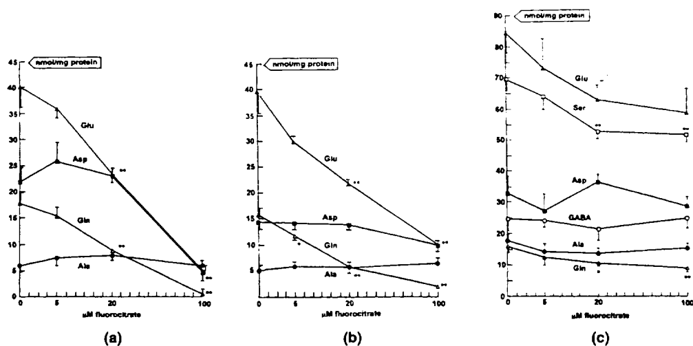
Fig. 1. (a and b): Intracellular levels of amino acids in cultured astrocytes after 24 hours of incubation with 0, 5, 20, or 100 \mu\text{M} fluorocitrate without addition of glutamine. Values are given as nmol/mg protein; means of five culture dishes per concentration of fluorocitrate; vertical bars indicate SEM. *: difference from control; * p < 0.05 ; **: p < 0.01 ; t -test. a: astrocytes from cerebral cortex; b: astrocytes from cerebellum. (c): Intracellular levels of amino acids in cerebellar neurons after 24 hours of incubation with 0, 5, 20, or 100 \mu\text{M} fluorocitrate and with 0.8 mM glutamine (as opposed to the 0.2 mM in Table I) in the incubation medium. Values are given as nmol/mg protein; means of five culture dishes per concentration of fluorocitrate; vertical bars indicate SEM. *: difference from control; * p < 0.05 ; **: p < 0.01 ; t -test.
