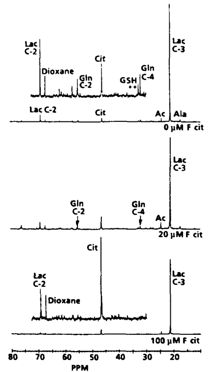
FIG. 2. 13 C spectra of the media of cultured astrocytes incubated for 22 h with 3 mM [1- 13 C]glucose and 3 mM [2- 13 C]acetate, without glutamine supplementation but with 0, 20, or 100 μM fluorocitrate (F cit). Insets: 10× magnifications of the corresponding spectra. Lac C-2 and Lac C-3, the C-2 and the C-3 of lactate; Gln C-2 and Gln C-4, the C-2 and the C-4 of glutamine; Cit, the sum of the signals from the C-2 and the C-4 positions in citrate; GSH++, glutathione and other glutamate-containing peptides; Ac, the C-2 of acetate; Ala, the C-3 of alanine.
