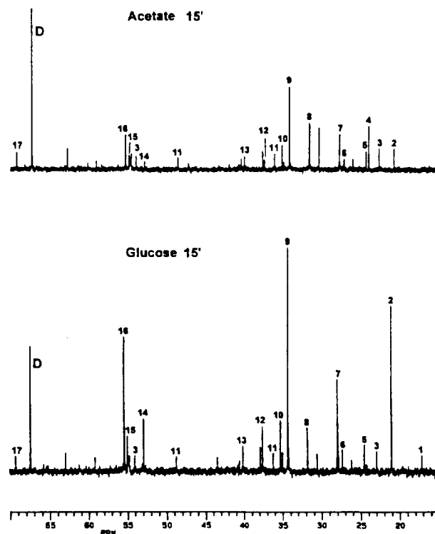
FIG. 1. ^{13}\text{C} NMR spectra of brain extracts from mice injected intravenously with [2-^{13}\text{C}] acetate (upper panel) or [1-^{13}\text{C}] glucose (lower panel) with survival for 15 min. Peak assignment was as follows: 1, alanine C-3; 2, lactate C-3; 3, N -acetylaspartate; 4, acetate C-2; 5, GABA C-3; 6, glutamine C-3; 7, glutamate C-3; 8, glutamine C-4; 9, glutamate C-4; 10, GABA C-2; 11, taurine; 12, aspartate C-3; 13, GABA C-4; 14, aspartate C-2; 15, glutamine C-2; 16, glutamate C-2; 17, lactate C-2; and D, dioxane (internal standard).
