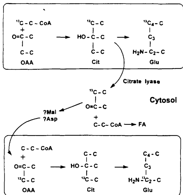
FIG. 5. The possible reactions leading to a higher ^{13}\text{C} enrichment of the C-2 than of the C-3 in glutamate (Glu) from [2- ^{13}\text{C} ]acetate: [2- ^{13}\text{C} ]Acetate is converted to [2- ^{13}\text{C} ]acetyl-CoA and [2- ^{13}\text{C} ]citrate ([2- ^{13}\text{C} ]Cit) in glia, which via the TCA cycle yields [4- ^{13}\text{C} ]Glu. With the next turn of the TCA cycle this label is distributed equally between the C-2 and C-3 in Glu (Fig. 1). [2- ^{13}\text{C} ]Cit may also leave the mitochondrion (rectangle) to undergo cleavage by Cit lyase in the cytosol, yielding [3- ^{13}\text{C} ]oxaloacetate ([3- ^{13}\text{C} ]OAA). This carbon skeleton may enter a mitochondrion, e.g., as malate (Mal) or aspartate (Asp), and will via the TCA cycle yield [4- ^{13}\text{C} ]Cit and hence [2- ^{13}\text{C} ]Glu. FA, fatty acids.
