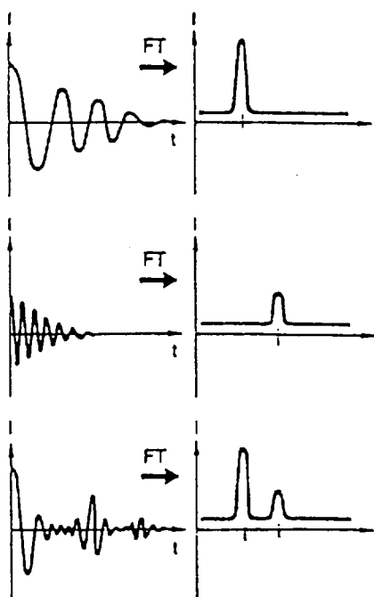
Figure 2.2 The precession frequency of a nucleus is Fourier transformed (FT) to yield a peak in an NMR spectrum (upper two panels). The lower panel shows the sum of the two upper frequencies and their transformation into two separate peaks in an NMR spectrum. The peak height is proportional to the signal intensity which (in the case of ^{13}\text{C} NMR) is proportional to the amount of ^{13}\text{C} in a specific carbon position, e.g. the amount of ^{13}\text{C} in the C-4 of glutamate or glutamine.
