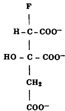
Figure 2.3 Fluorocitrate
