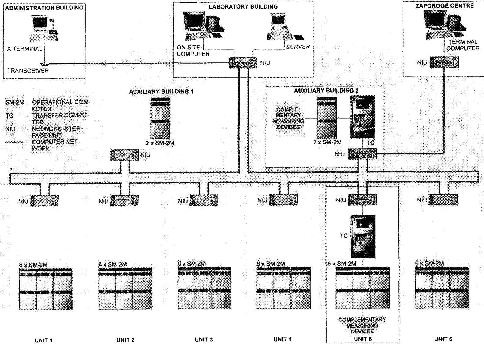
Figure 2 The structure of the technical system at Zaporozh'ye NPP site to improve the operational monitoring
