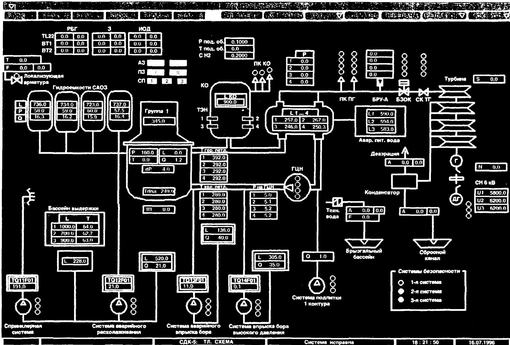
Figure 4 Technological scheme for the representation of the actual operational parameters at the 5-th unit of Zaporozhye NPP
