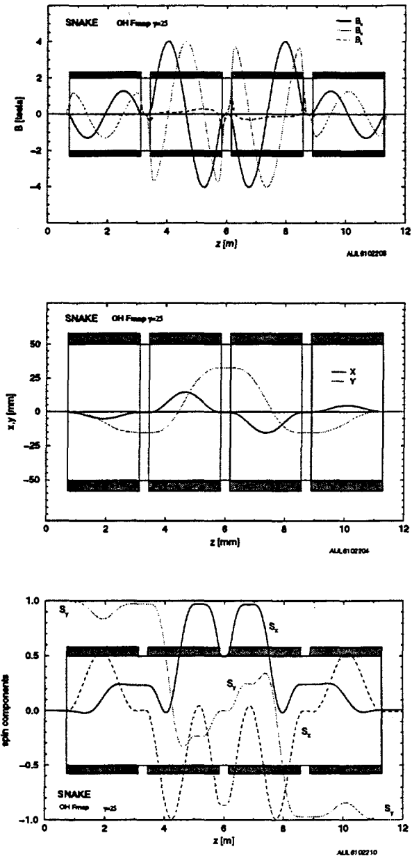
Figure 1: Magnetic field, 25 GeV proton trajectory, and proton spin components versus distance through a RHIC Siberian Snake.
