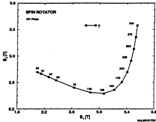
Figure 2: Spin Rotator field strengths for various RHIC beam energies.
