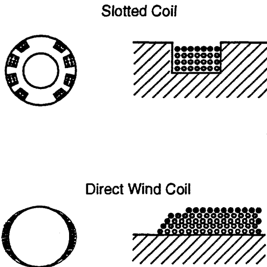
Figure 3: Possible Magnet Technologies.
