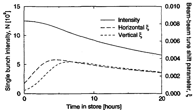
Figure 5: Beam-beam tune shift parameter evolution.
