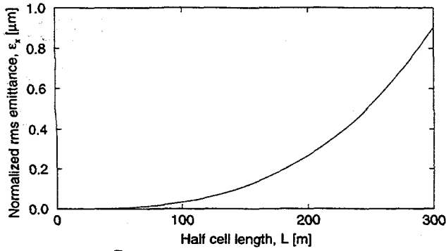
Figure 1: Equilibrium emittance versus half cell length
