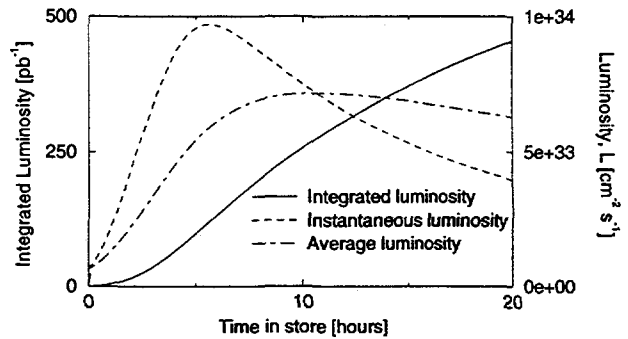
Figure 3: Luminosity evolution during a 20 hour store.
