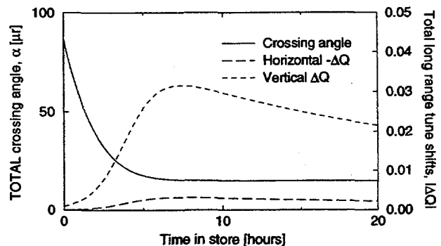
Figure 6: Long range tune shift evolution, per IR.
