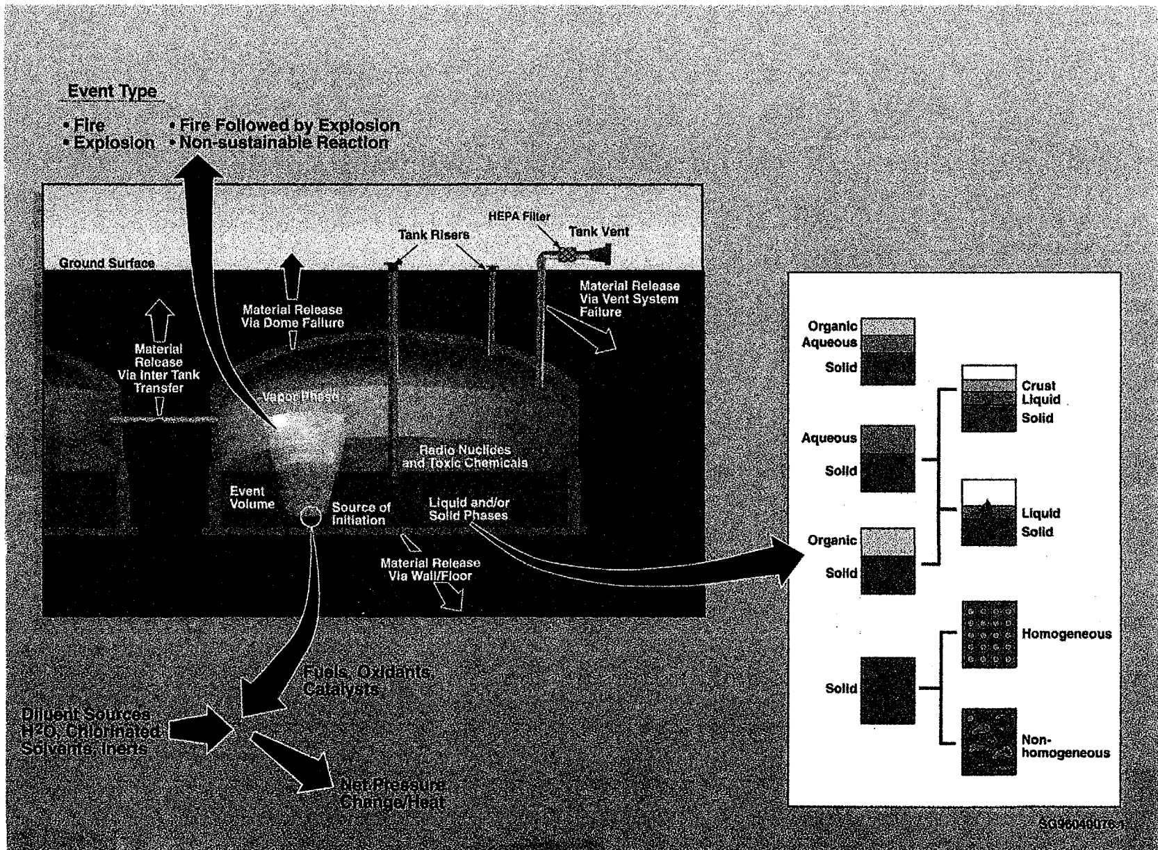
Figure 2.1. Conceptual Model of an Event Involving Organic-Bearing Waste
