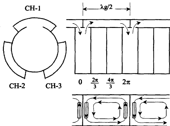
Fig. 2 Schematic structure
