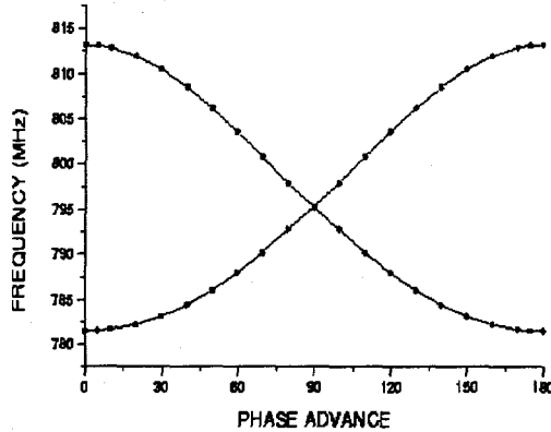
Fig.4 The dispersion curve
