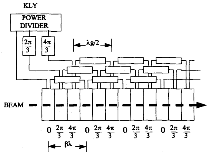
Fig.1 The principle diagram
