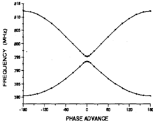
Fig.5 Two pass band not matched
