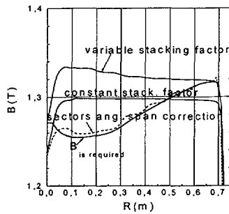
Figure 9: Radial dependence of the average magnetic field
