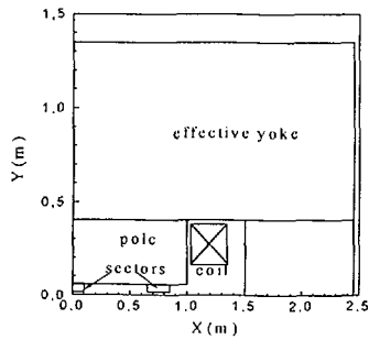
Figure 2: The view of the X-Y model for the cyclotron IC-35 magnet ( R=0.5 m)
