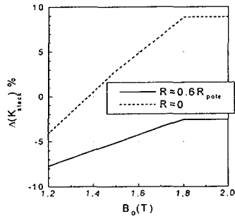
Figure 7: Relative correction of the sector stacking factor
