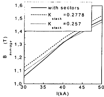
Figure 6: Average field dependence on the excitation current, R=0.5 m
