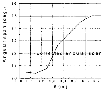
Figure 10: Radial variation of the sector angular span
