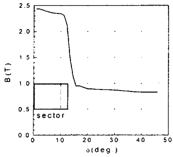
Figure 4: Azimuth magnetic field distribution for R=50 cm, \alpha=25^\circ
