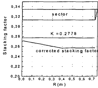
Figure 8: Radial dependence of the sector stacking factor
