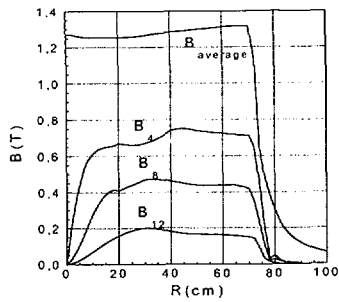
Figure 3: Magnetic field characteristics for the sector angular span \alpha=25^\circ
