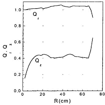
Figure 5: Frequencies of radial and axial free betatron oscillations
