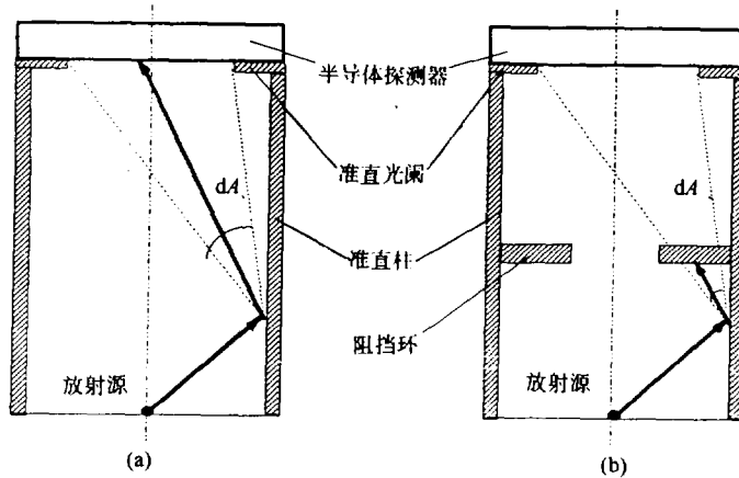
图3 \alpha 壁散射及减小壁散射影响的方法 Fig. 3 \alpha Scattering from the wall of the cylindrical chamber and the method used to deduce the scattering
