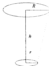
图 2 准直光阑对源所张的立体角 Fig. 2 Solid angle subtended by the aperture
