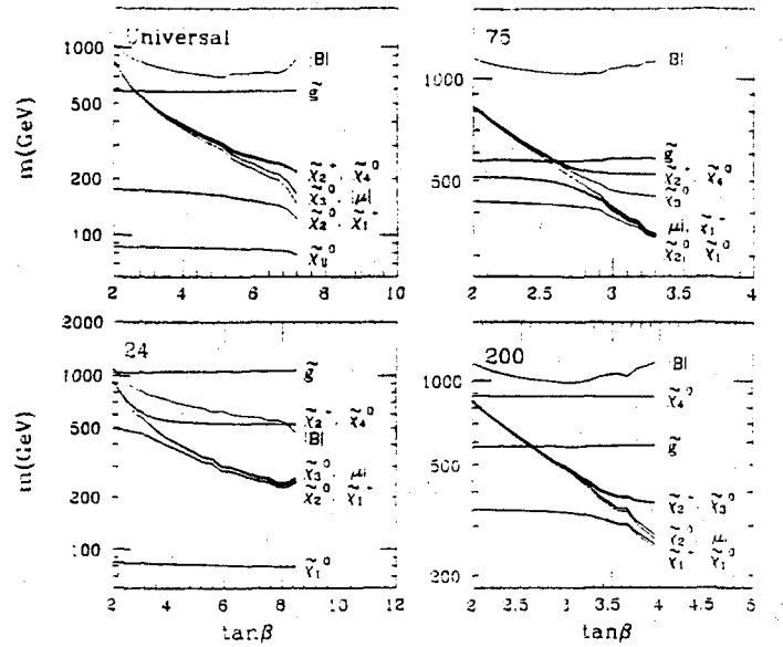
Figure 3: Physical (pole) gaugino masses as a function of \tan \beta for the 1 (universal), 24, 75, and 200 F representation choices. Also plotted are |B| and |\mu| . We have taken m_0 = 1 TeV and M_3 = 200, 400, 200, 200 GeV, respectively.
