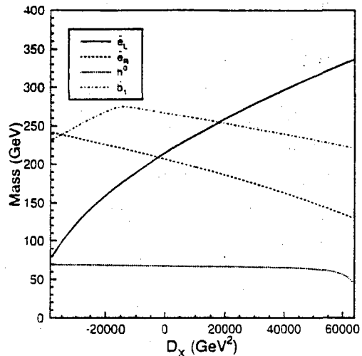
Figure 1: Mass spectrum as a function of D_X .
