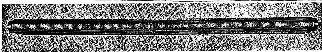
A fuel element with the end spiders removed. Enclosing a natural-uranium slug in a helium atmosphere, the magnesium alloy tube is turned from the solid with a single-start helical fin of \frac{1}{8} -in. pitch. Transverse fins have superior heat-transfer properties under the reactor conditions than have longitudinal ones.
