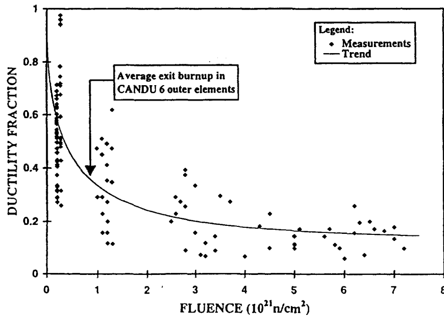
(b) Effect of Neutron Damage (Source: Tayal et. al, 1995)
