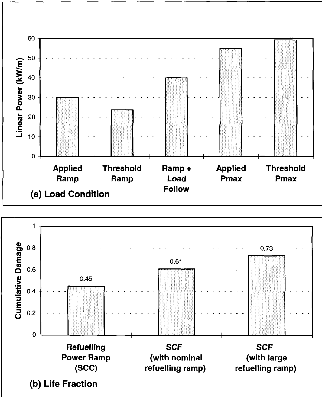
Figure 6: Fatigue Life of Bruce Fuel: Weekly Cycles
