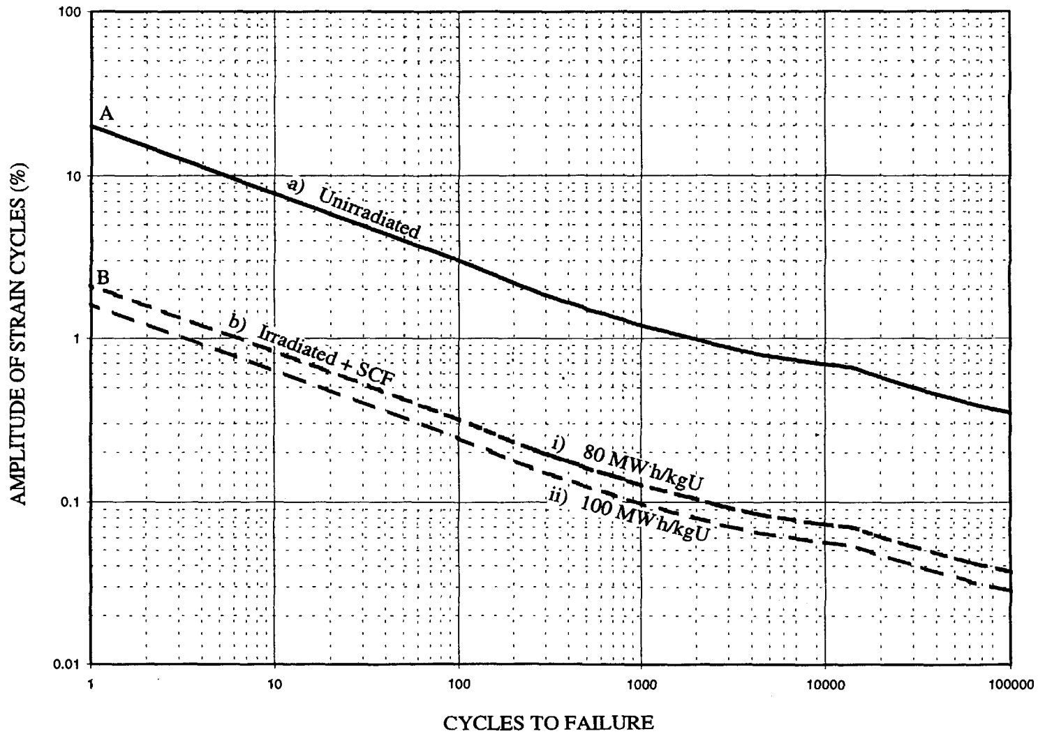
Figure 3: Effect of Corrosive Environment and Irradiation on the Fatigue Life of Zircaloy
