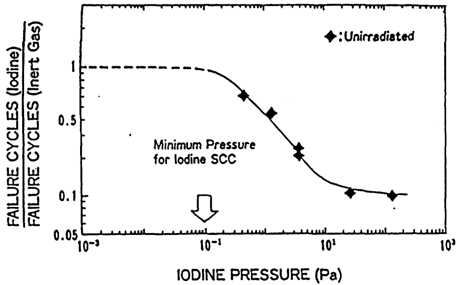
(a) Effect of Iodine Concentration (Source: Nakatsuka et. al, 1991)
