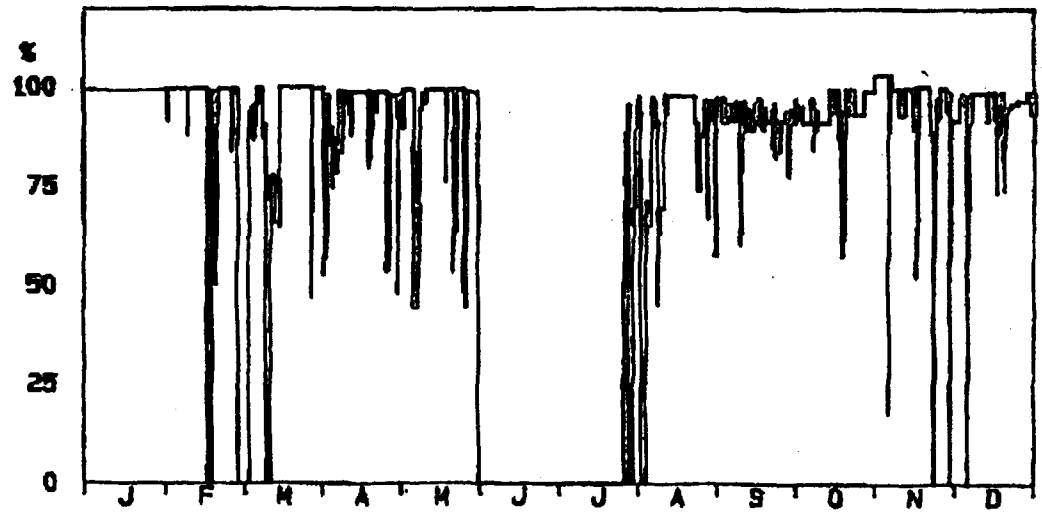
Figure 1: 1986 Bruce B Unit 6 Concentrations of ^{131}\text{I} , ^{88}\text{Kr} and ^{135}\text{Xe} in Coolant ( \mu\text{Ci}/\text{kg} , top) and Reactor Power (bottom)
