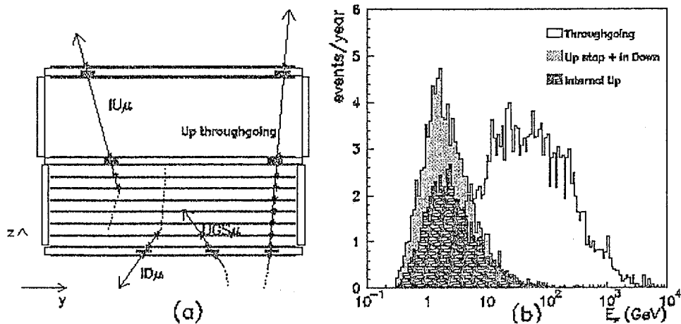
Fig. 1. a) Sketch of different event topologies induced by neutrino interaction in or around MACRO. IUμ= Internal Upgoing muons; IDμ= Internal Downgoing muons; UGSμ= Upgoing Stopping muons; Up-throughgoing = Upward throughgoing muons. In the figure, the stars represent the streamer tube hits, and the black boxes the scintillator hits. The T.o.F. of the particle can be measured for the IUμ and Up-throughgoing events. b) Parent neutrino energy distribution for the three \nu_\mu samples.
