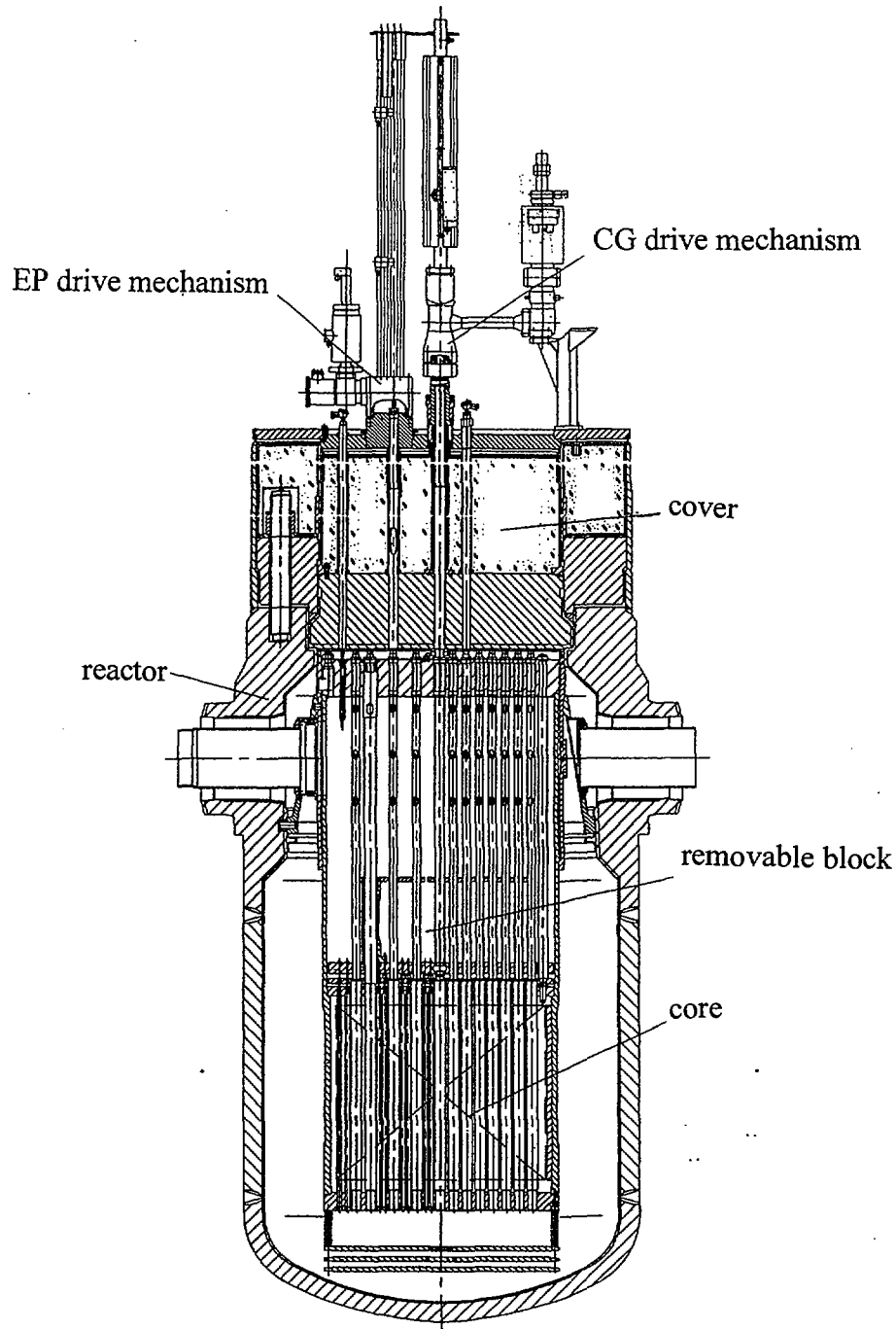
Fig.1. Reactor
