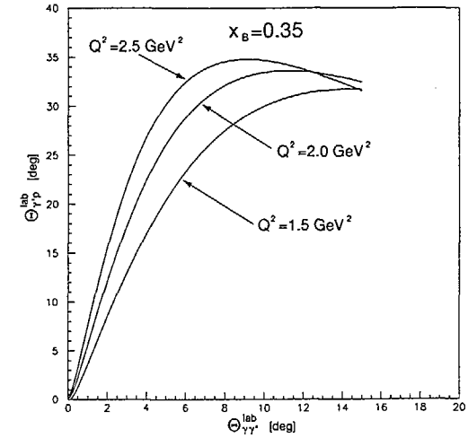
Figure 8: Relation between \theta_{\gamma\gamma^*} (angle between the emitted photon and the virtual photon) and \theta_{\gamma p} (angle between the virtual photon and the recoil proton) in the laboratory frame. The experimental acceptance is illustrated in Fig. 5.
