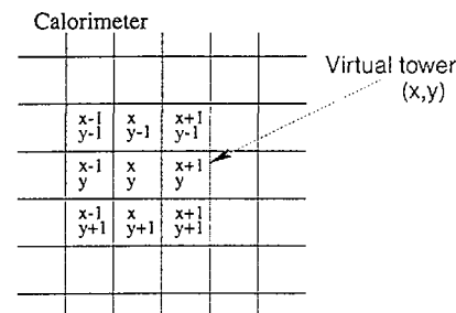
Figure 16: Definition of a virtual tower at coordinates (x, y) in the calorimeter, composed of 9 blocks (the central block + the first ring around it).
