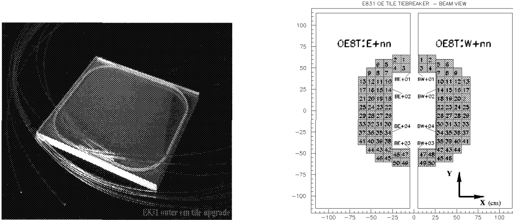
Figure 4: left) A complete tile counter before wrapping; right) layout of tile counter array, and edge counters.
