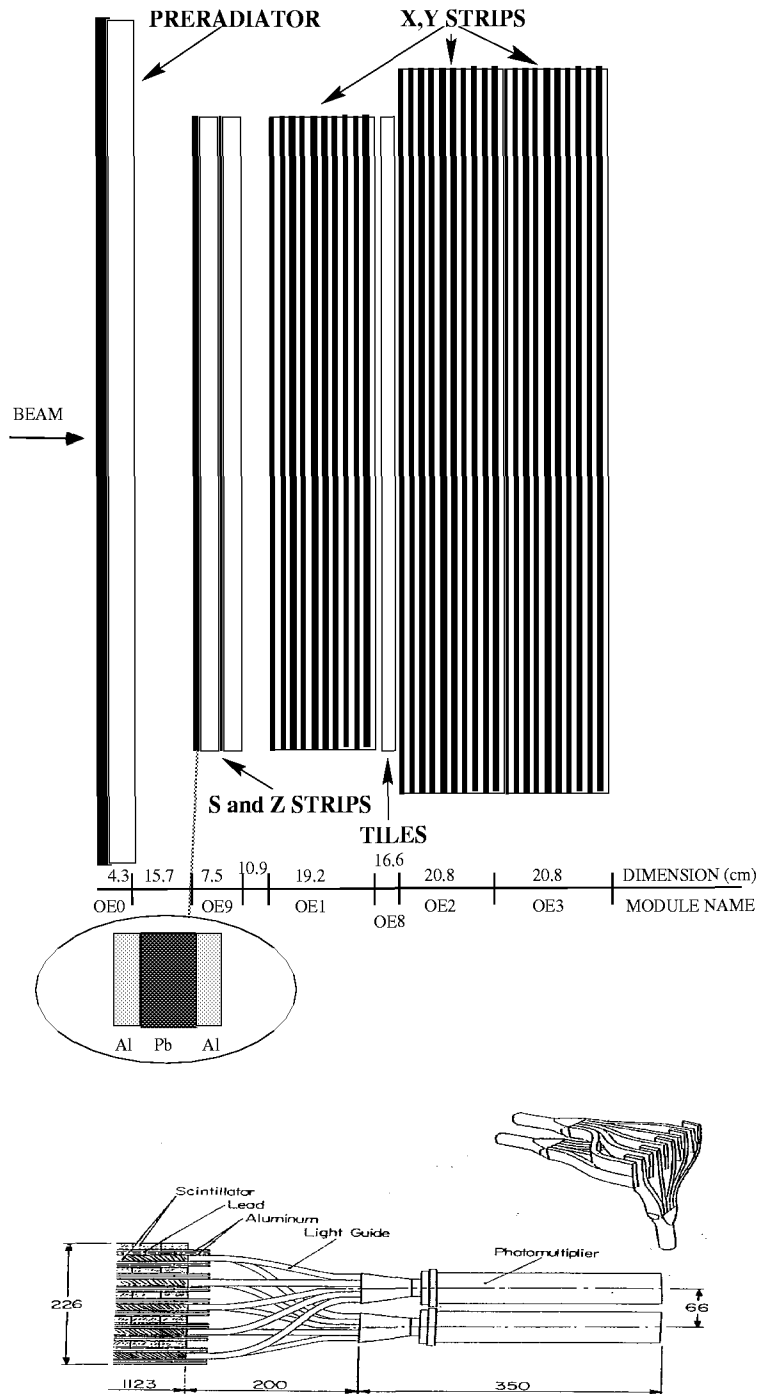
Figure 2: a) The Outer em calorimeter longitudinal structure showing the sandwich of absorber and scintillator planes. b) X and Y strip planes interlaced and five-fold integrated to a readout PMT (dimensions are millimeters).
