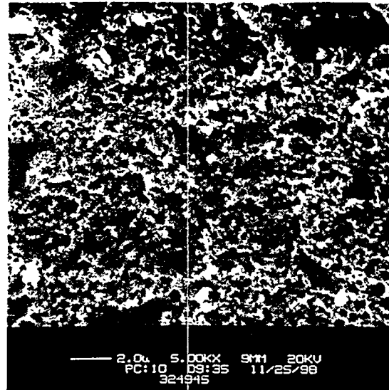
(a) Atomized U-10Mo
