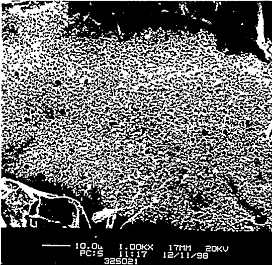
(b) Ground U-6Mo-0.6Ru
