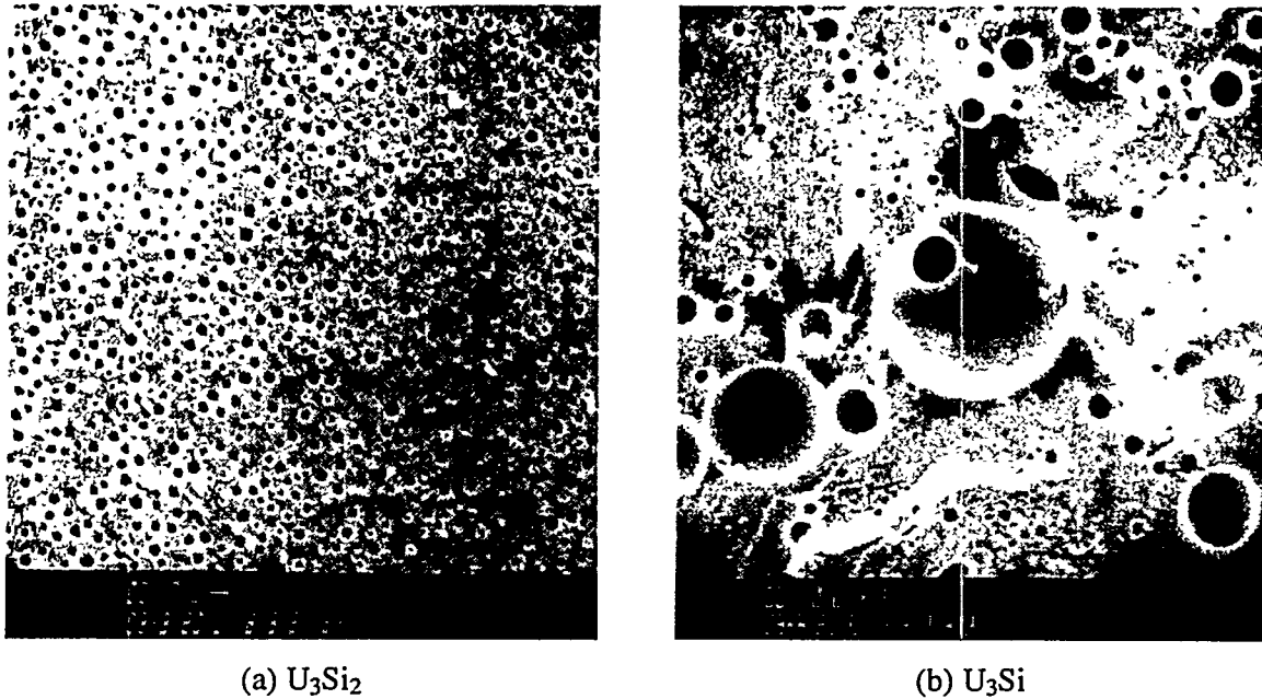
Fig. 1. Examples of stable (a) and unstable (b) fission-gas-bubble morphologies.
