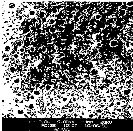
(a) U-10Mo
