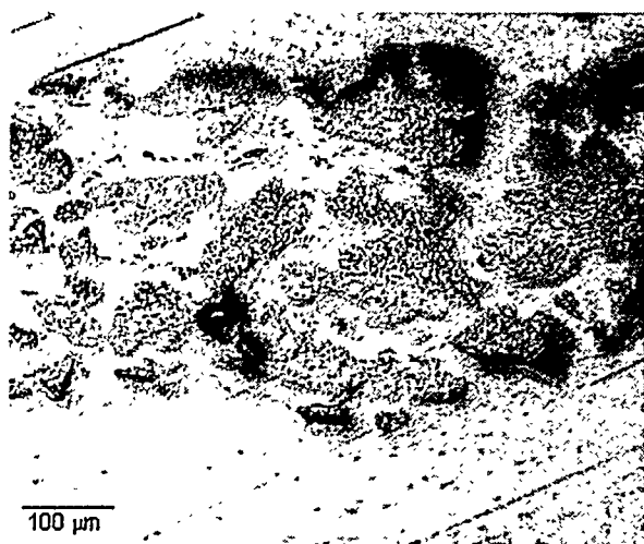
(a) U-6Mo at ~70% burnup
