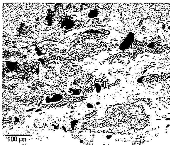
(b) U-5Nb-3Zr at ~40% burnup
