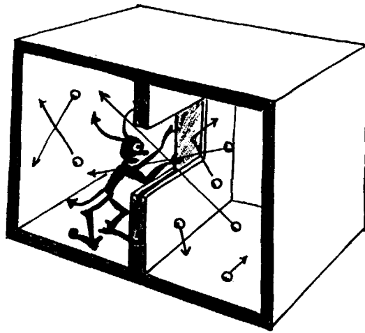
Fig.10 Maxwell's demon (reproduced from [9]).
