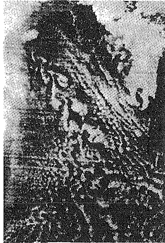
Fig.3 An example of Karman-vortex-like structure in clouds. Clouds near Kyushu island are shown. (Quoted from [2]).
