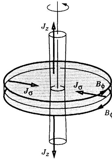
Fig.12 A model of accretion disk (quoted from [4]).
