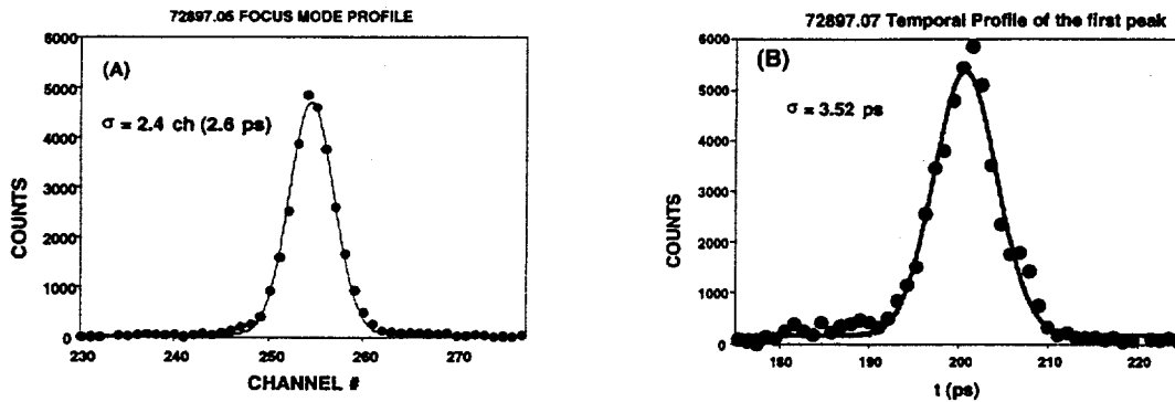
FIGURE 4. Streak camera images taken with a 550 x 40 nm bandpass filter for the focus mode (a) and the R2 streak range (b). The total observed bunch length is about 3.6 ps ( \sigma ) from the conventional gun and buncher system.
