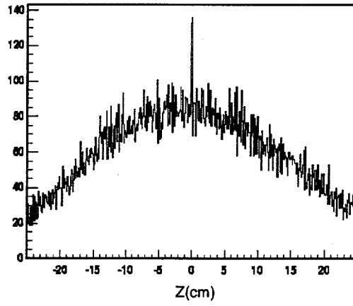
Figure 4: Vertex reconstruction in PHOBOS.
