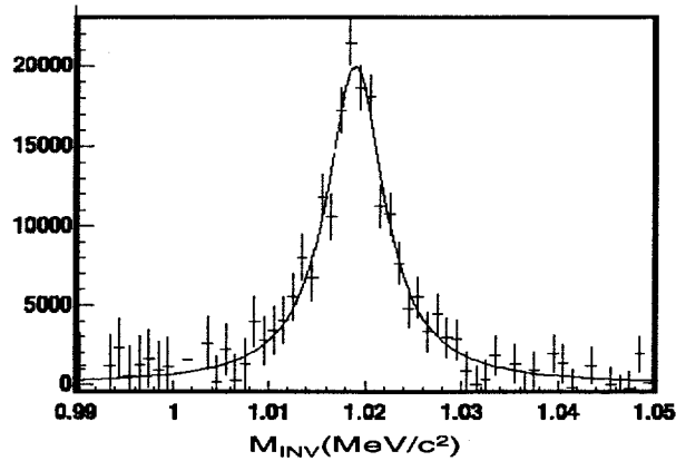
Figure 6: Phi-meson reconstruction in PHOBOS.
