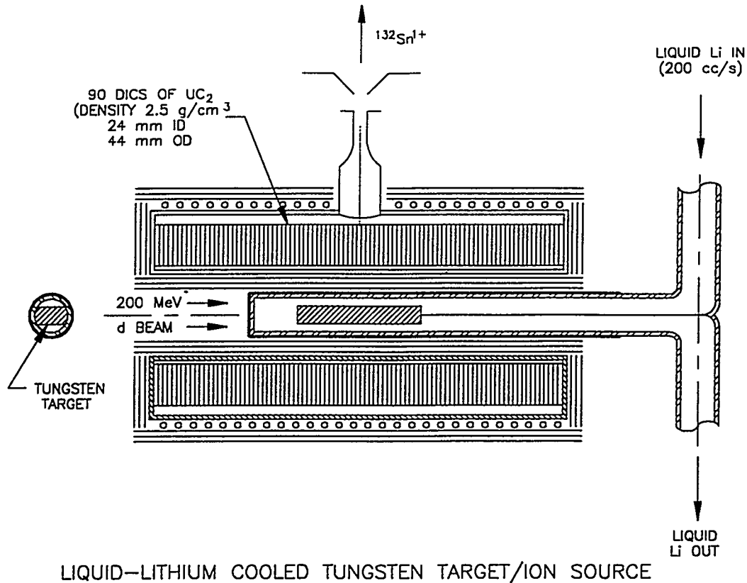
Figure 3. Schematic of a two-step, neutron-generator-type, high-power target for the production of fission fragments. A deuteron beam on a tungsten primary target produces secondary neutrons. Circulating liquid lithium cools the primary target. The secondary uranium carbide target is heated to 2000 C by a combination of the fission power and supplemental electrical power.
