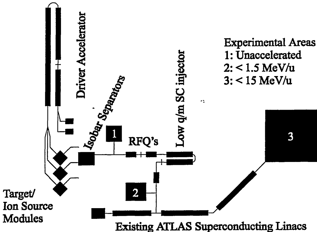
FIGURE 1. A block diagram of the proposed Advanced ISOL Facility based on ATLAS at Argonne. The major components of the complex, including the three different experimental areas, are indicated. The details of the low energy beam switchyard that connects the three target modules to the various experimental areas and/or post accelerators are not shown.
