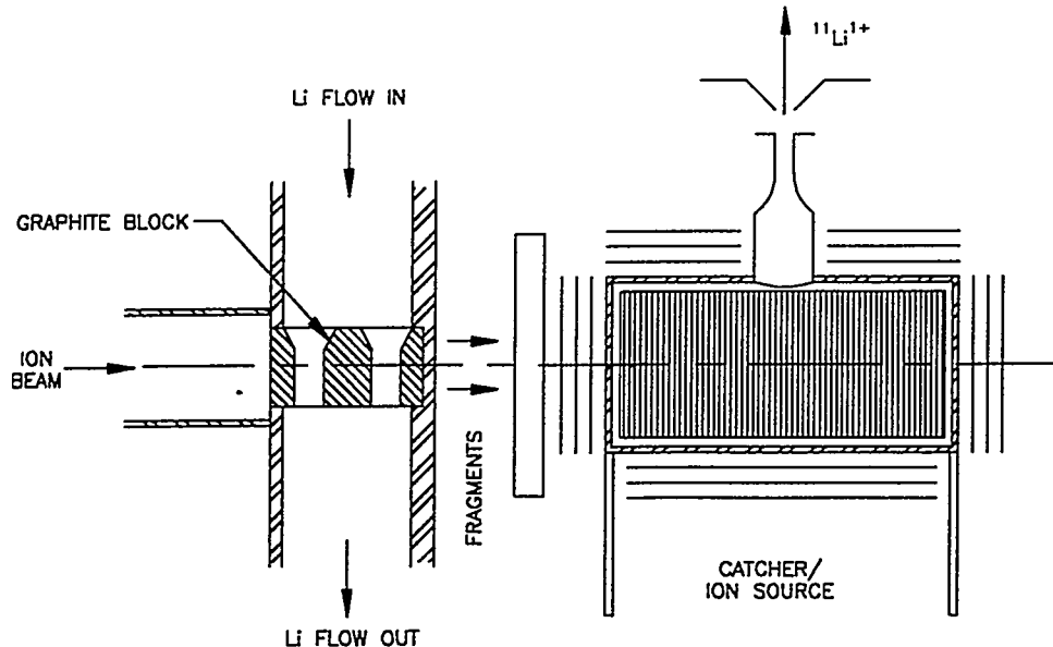
Figure 4. Schematic of a two-step, fragmentation/catcher target combination. A high-power, neutron-rich heavy ion beam, such as ^{18}\text{O} , stops in the primary target that consists of a combination of graphite and liquid lithium coolant. The neutron-rich, lower-Z fragments, such as ^{11}\text{Li} , have a much longer range than the primary beam and are stopped in the downstream catcher. The catcher is close-coupled to the ion source and is optimized for rapid release of the short-lived fragments.
