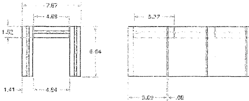
Figure 2: Ferrite blocks of injection kicker (dimensions in cm)
