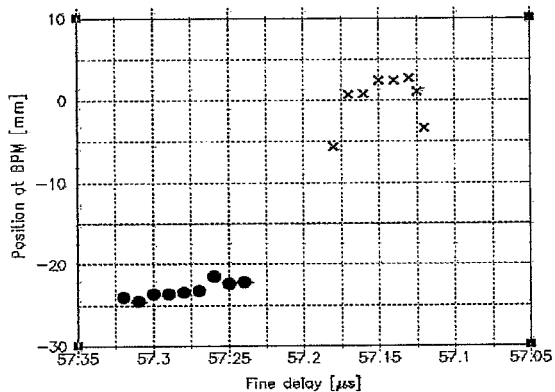
Figure 8: Beam based rise time measurement of the blue ring with one all-ferrite kicker magnet.
