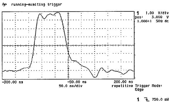
Figure 4: Current in the all-ferrite magnet (32 kV and 16Ω)
