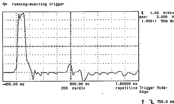
Figure 5: Current in the all-ferrite magnet (32 kV and 16 Ω)
