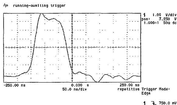
Figure 3: Current in the load of a dielectric kicker (30 kV into 16 \Omega ; scale 200A/V).
