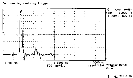
Figure 6: All-ferrite magnet with 25 Ω load @ 38 kV
