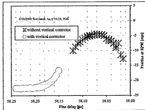
Figure 7: Beam based rise time and flat top measurement of the dielectric loaded kickers.
