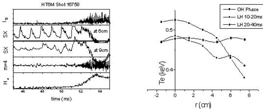
Fig.3 Deterioration of the confinement by MHD. Fig.4 T_e profiles before and during LHW
