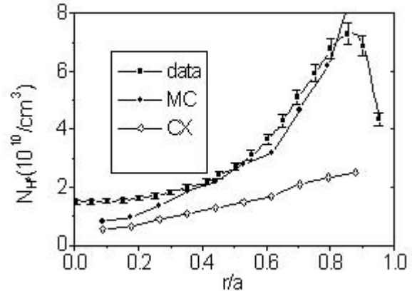
Fig.6 Monte-Carlo simulation
