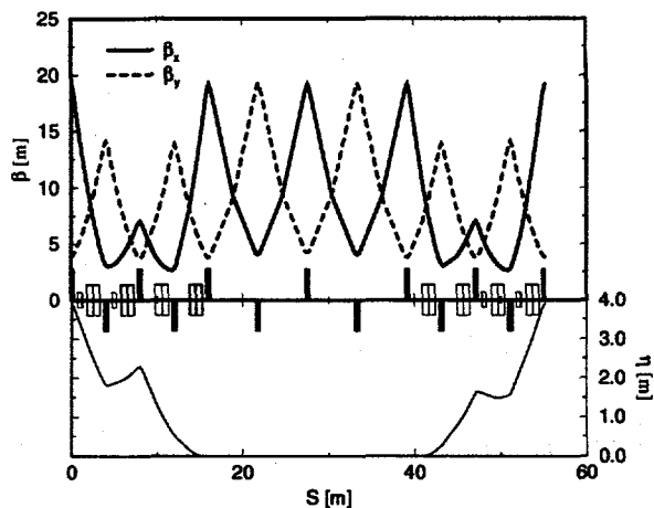
Figure 1: Split-tune FODO lattice.
