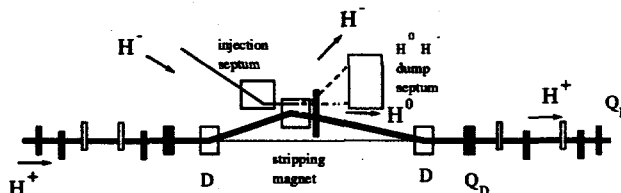
Figure 2: Foil injection in nominal FODO lattice.
