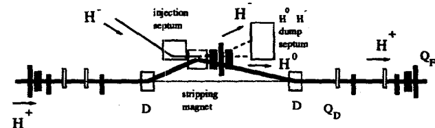
Figure 6: Doublet straight with foil injection.
