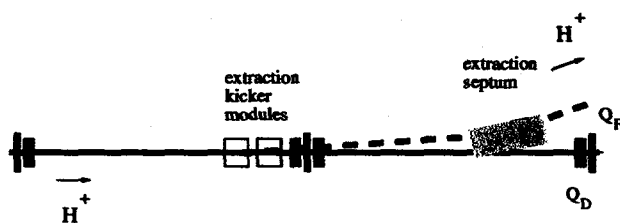
Figure 9: Extraction scheme for the hybrid lattice.
