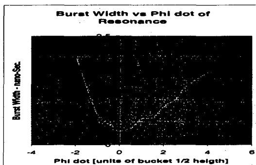
Fig 2. Burst Width as Function of Momentum.
