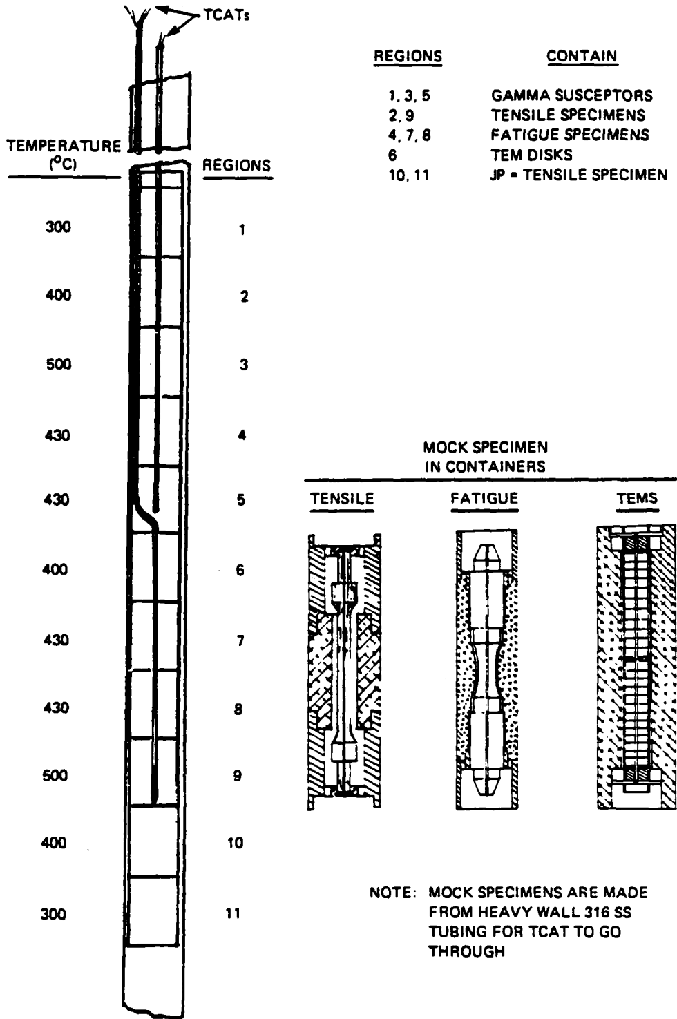
Fig. 4. General configuration of TTT capsule.
