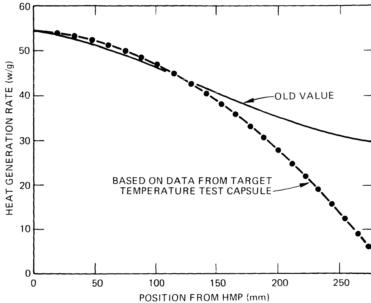
Fig. 3. Heat generation in HFIR target region (data is for 100 MW and should be multiplied by 0.85 to obtain present values).
