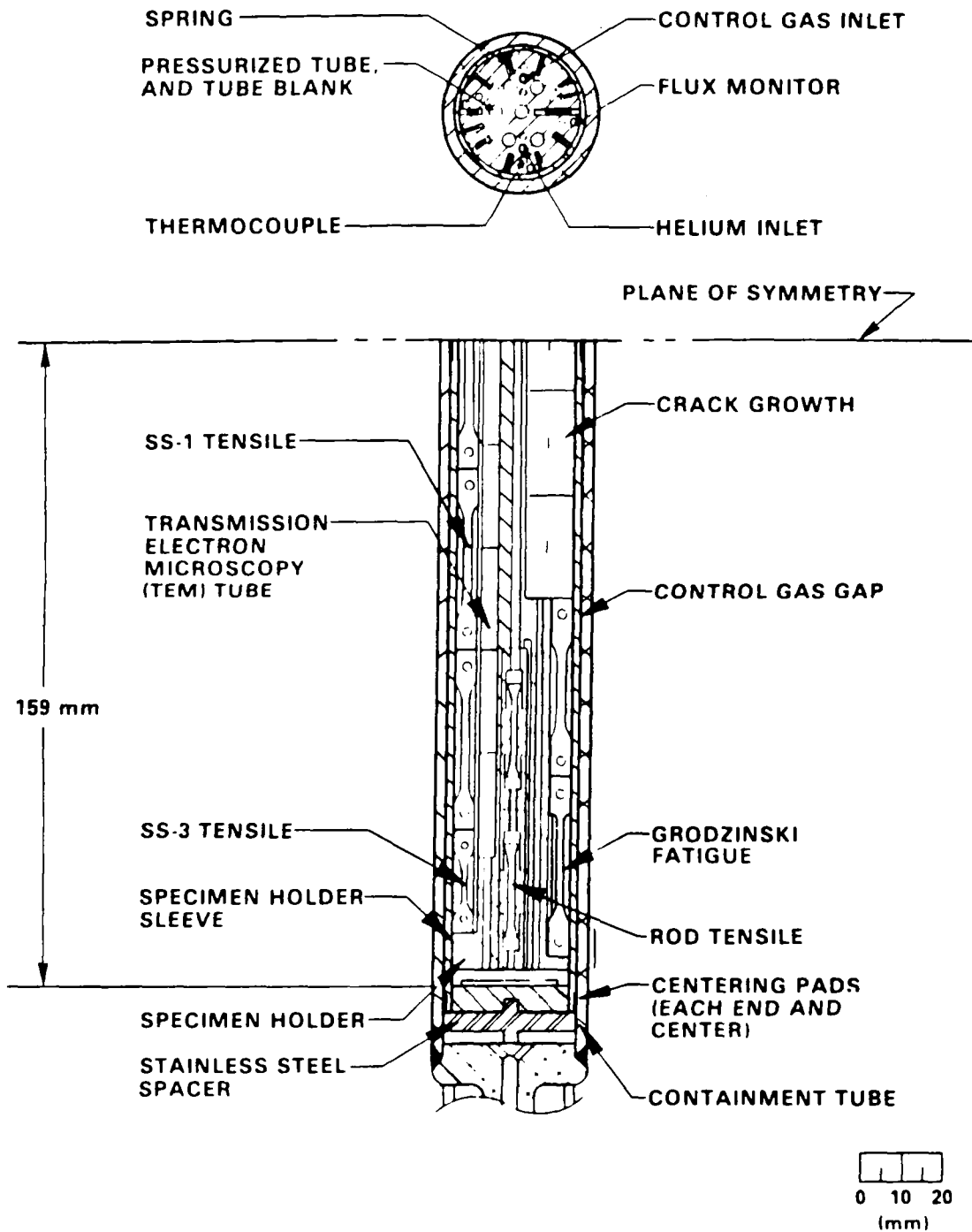
Fig. 5. Lower half of the HFIR-MFE-330J-1 capsule.
