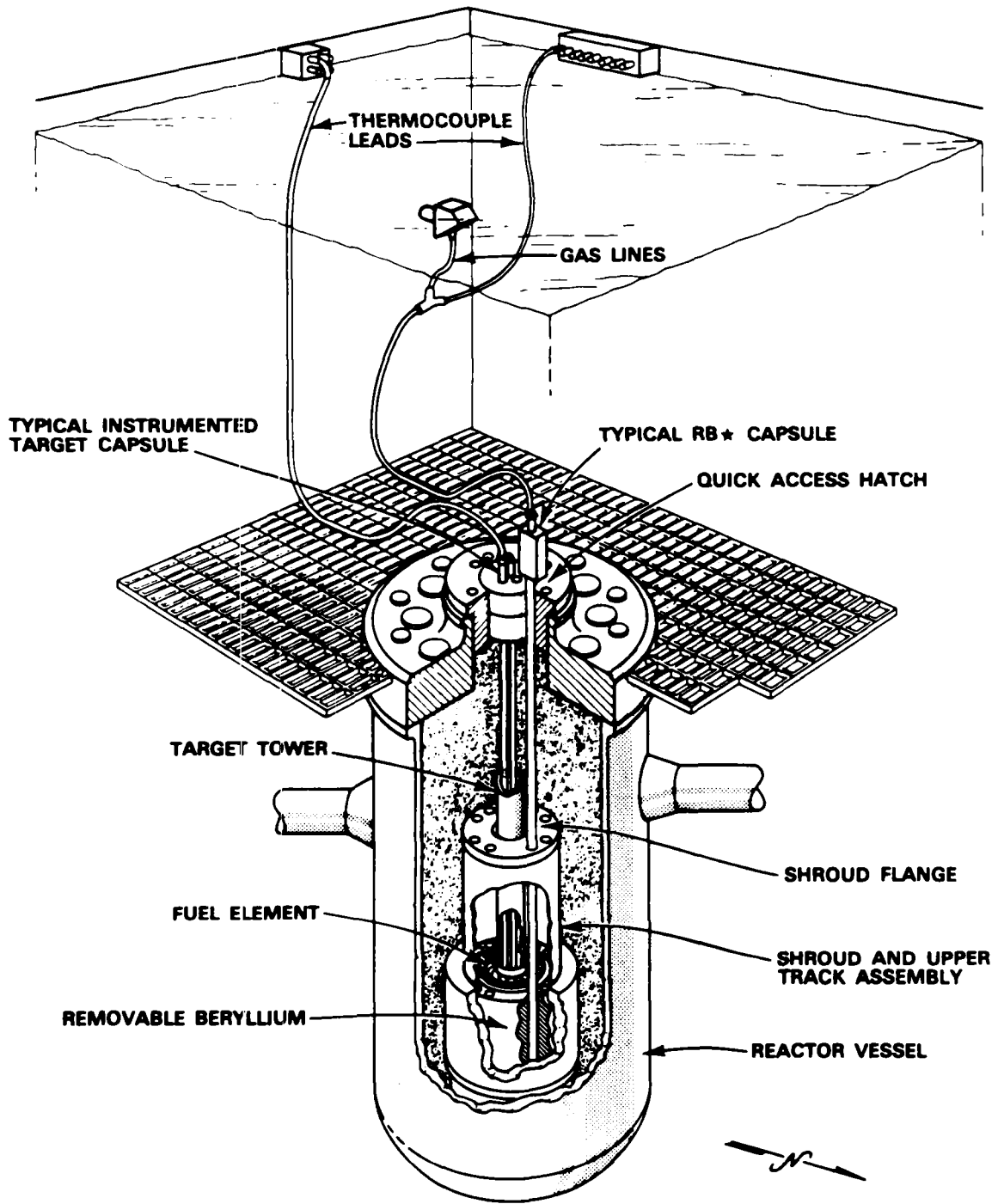
Fig. 1. The High Flux Isotope Reactor (HFIR).
