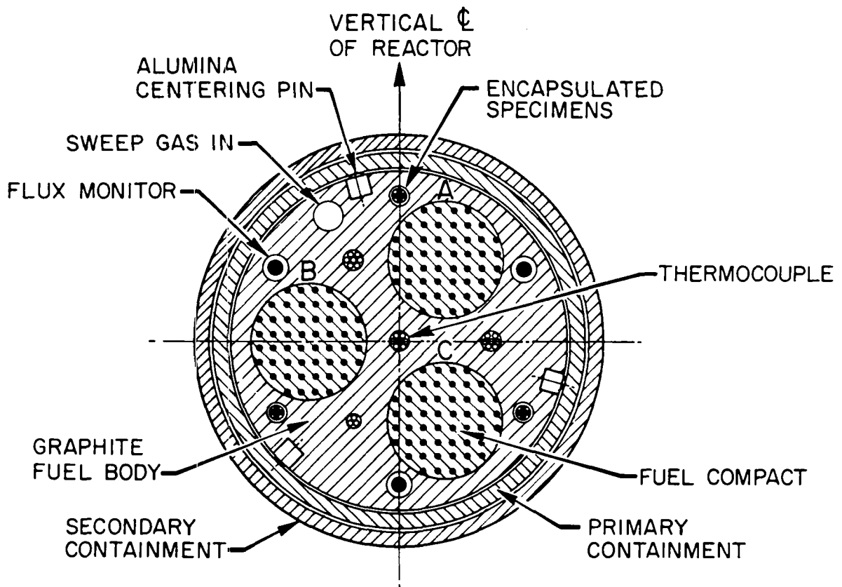
Fig. 6. Horizontal section through irradiation capsule HRB-21.
