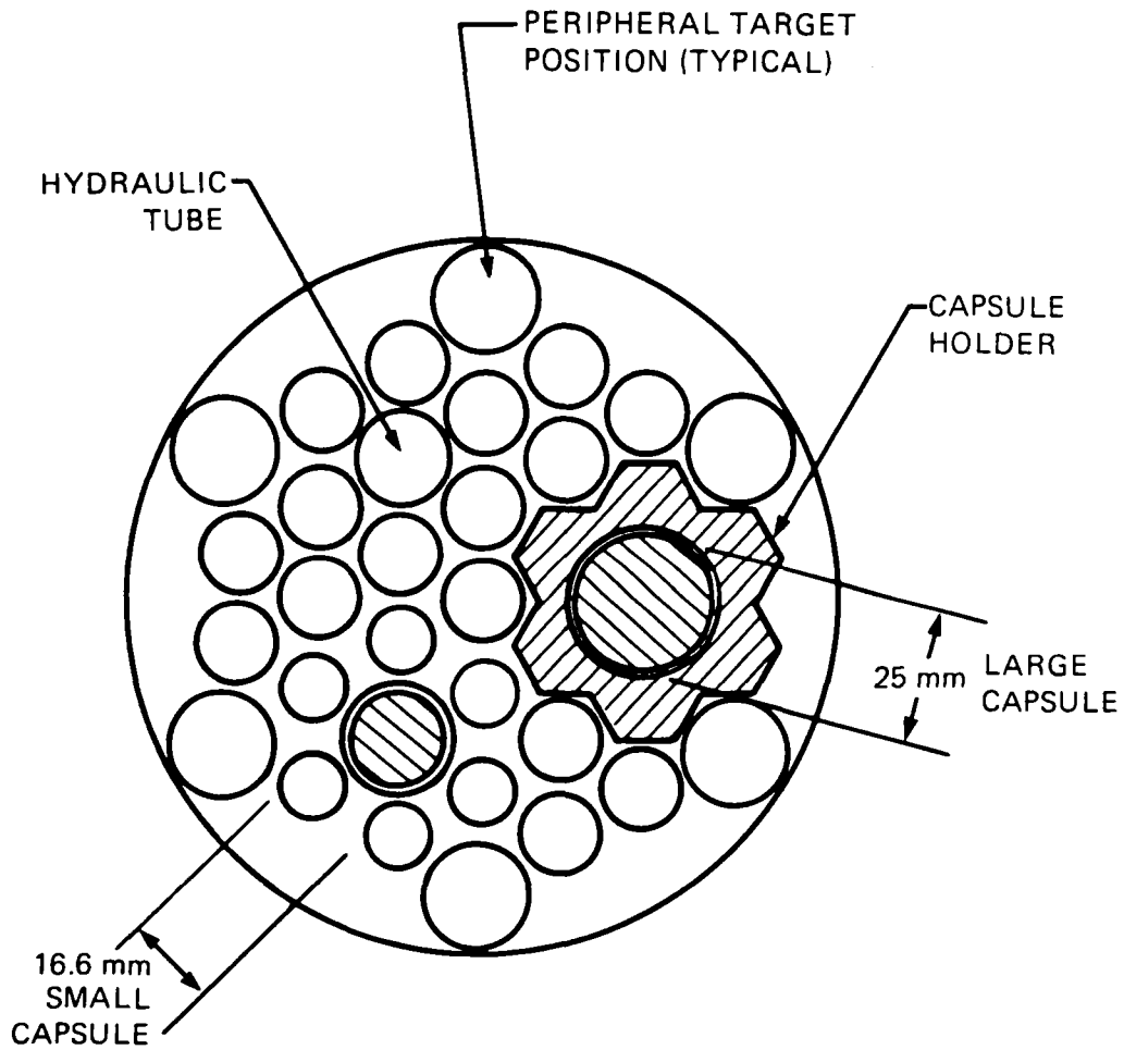
Fig. 2. Instrumented target positions illustrating capability of accommodating 25-mm capsules.
