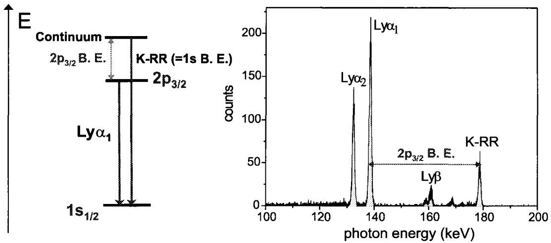
FIG. 2: Left side: schematic presentation of the Ly-\alpha_1 ( 2p_{3/2} \rightarrow 1s_{1/2} ) and K-RR transitions in a hydrogen-like ion; Right side: X-ray spectrum accumulated with a condition on the coincidence time (see above).
