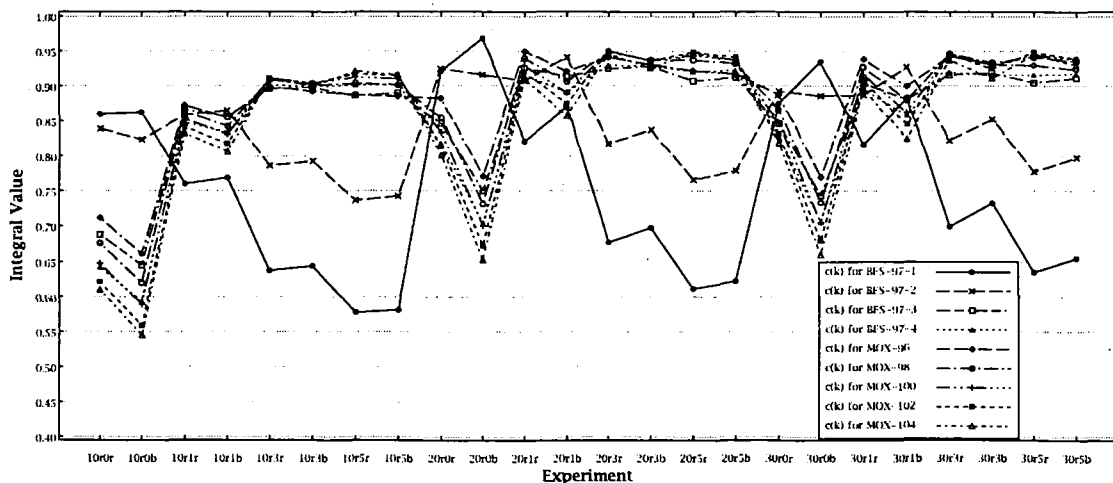
Fig. 4 Values of c_k for proposed experiments compared to reactor-grade applications.
