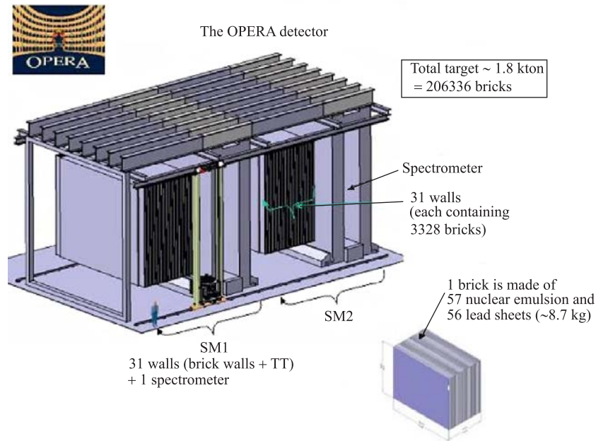
Fig. 1. General view of the OPERA setup
