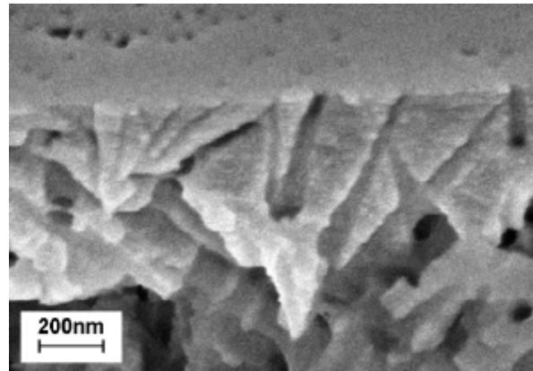
Fig.4. The fractures of PET asymmetric membrane after 90 h UV irradiation.
