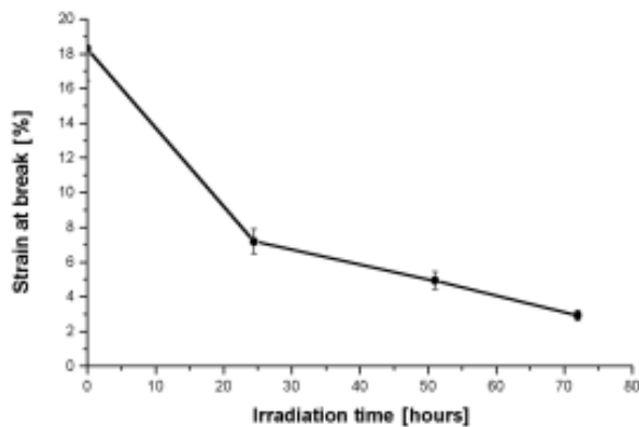
Fig.3. The strain at break of PET membrane – results of the tensile measurements vs. the UV irradiation time.
