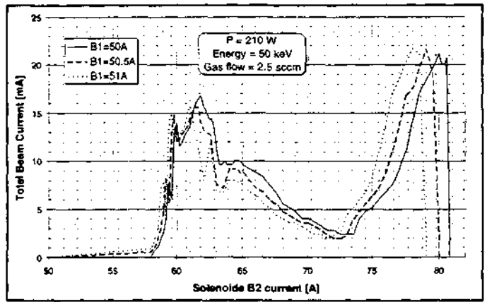
Figure 6: Extracted beam total current on DC toroid versus axial magnetic field.
