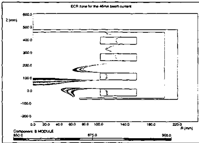
Figure 5 : Magnetic field calculation for the 46 mA extracted beam. The ECR area is located near the microwave injection.
