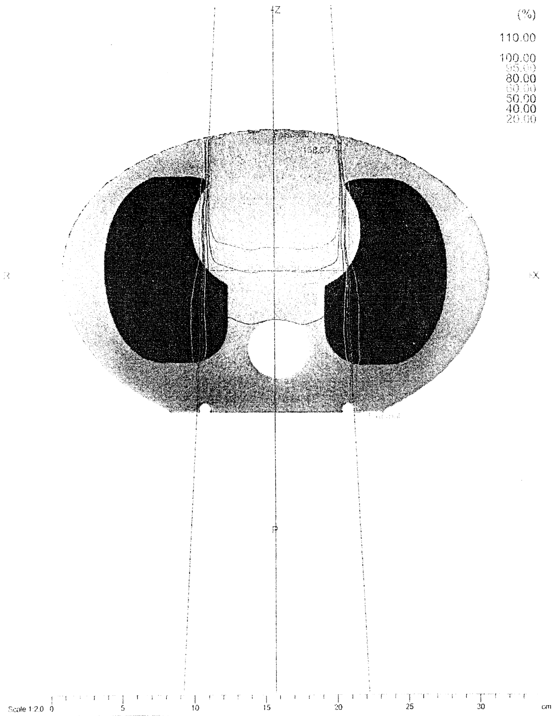
Figure 2 : calcul OMP en Collapsed-cone Convolution
