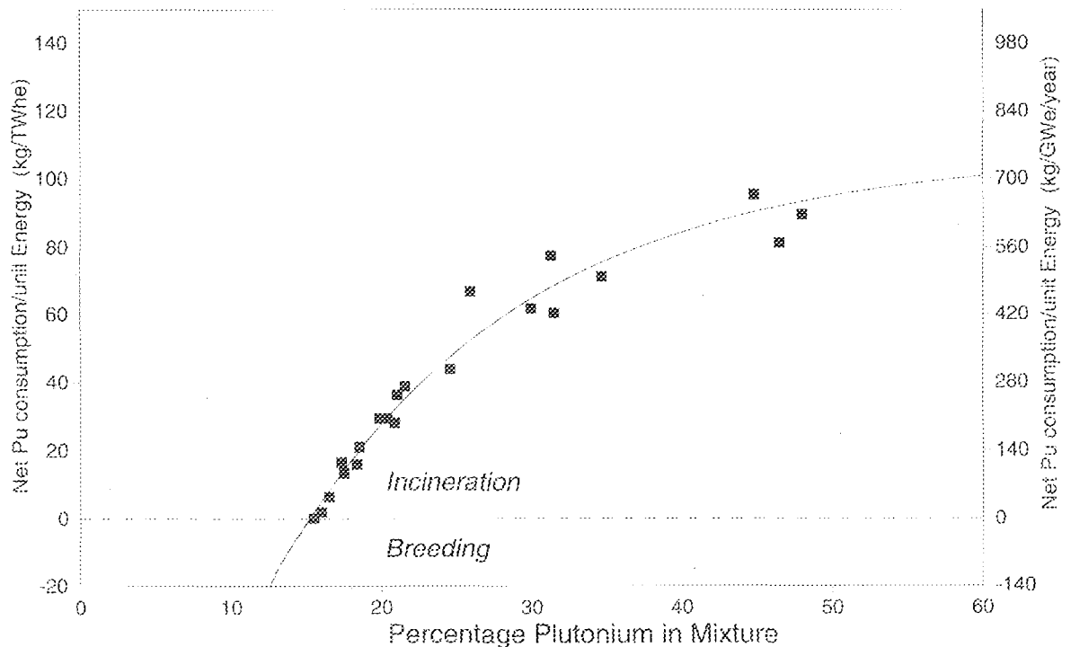
Figure 7a: Net plutonium consumption per unit energy in a uranium-plutonium fast breeder (CAPRA [5]) as a function of plutonium concentration. Note that the unit is kg/TW_e electric and not thermal.
