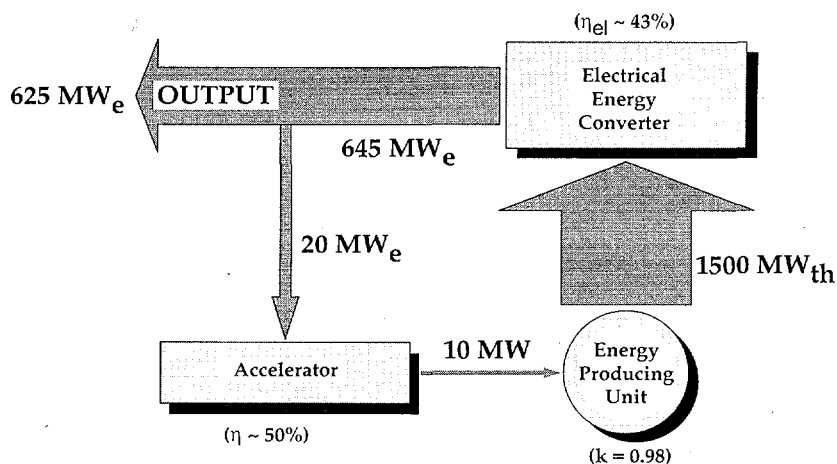
Figure 6: The energy amplification scheme in the standard EA system as proposed in Ref. [1].
