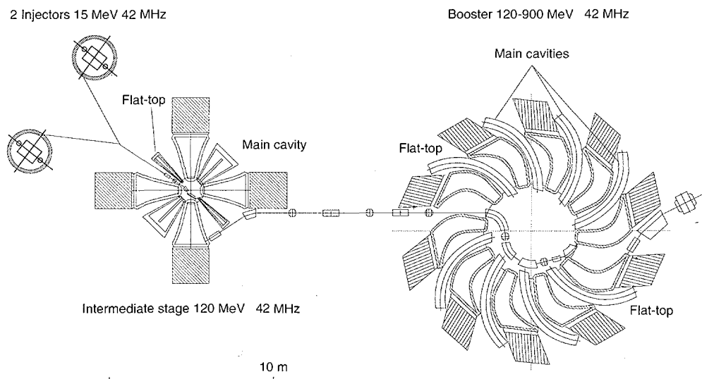
Figure 5: The full cyclotron high intensity accelerator layout proposed to drive a k = 0.98 EA [1].
