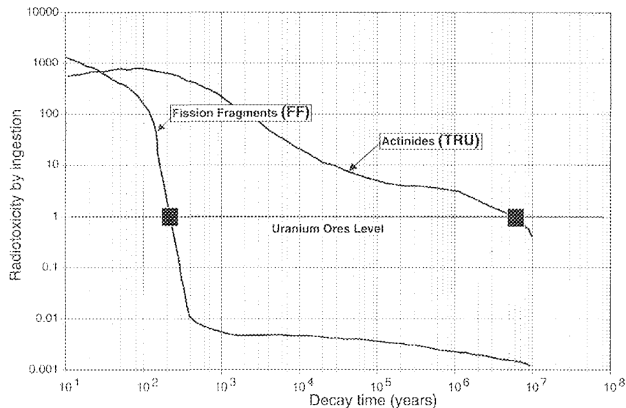
Figure 1: Time evolution of the potential radiotoxicity (relative to uranium ore) of the two main components of nuclear waste for PWR spent fuel, obtained with the ORIGEN2 code, with updated radiotoxicity data.
