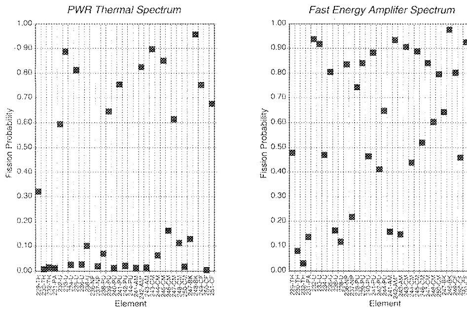
Figure 3: Comparison of fission and capture probabilities of actinides for thermal and fast neutron fluxes.
