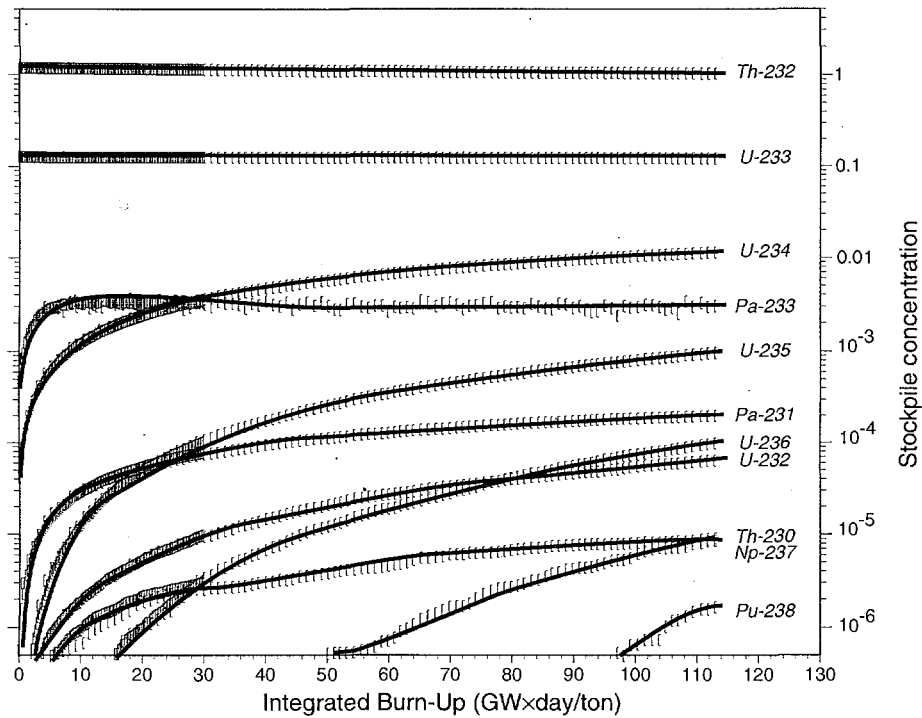
Figure 7b: Evolution as a function of burnup of the stockpile of the main elements present in the EA fuel.
