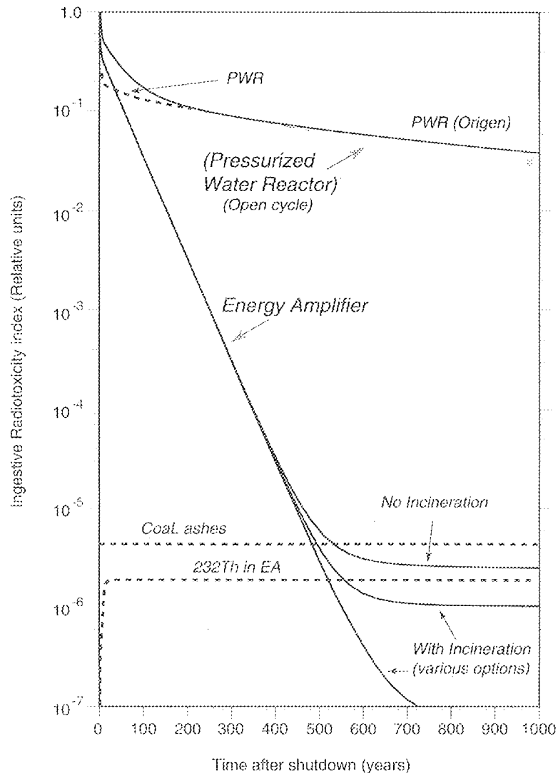
Figure 8: Evolution of the potential radiotoxicity of nuclear waste for PWR, EA and coal burning power station, showing that in the EA, the long term radiotoxicity can be 4 orders of magnitude smaller than in a PWR in open cycle and is dominated by LLFF if no further incineration is performed (adapted from Ref. [8]).
