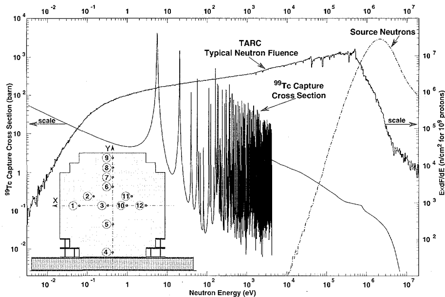
Figure 9: This figure illustrates the Adiabatic Resonance Crossing principle, showing how the presence of lead, transforms the spallation neutron energy distribution into a flux of slowing down neutrons, with iso-lethargic steps smaller than the width of cross section resonances where they will certainly be captured. A sketch of the 334 ton TARC lead assembly is also shown.
