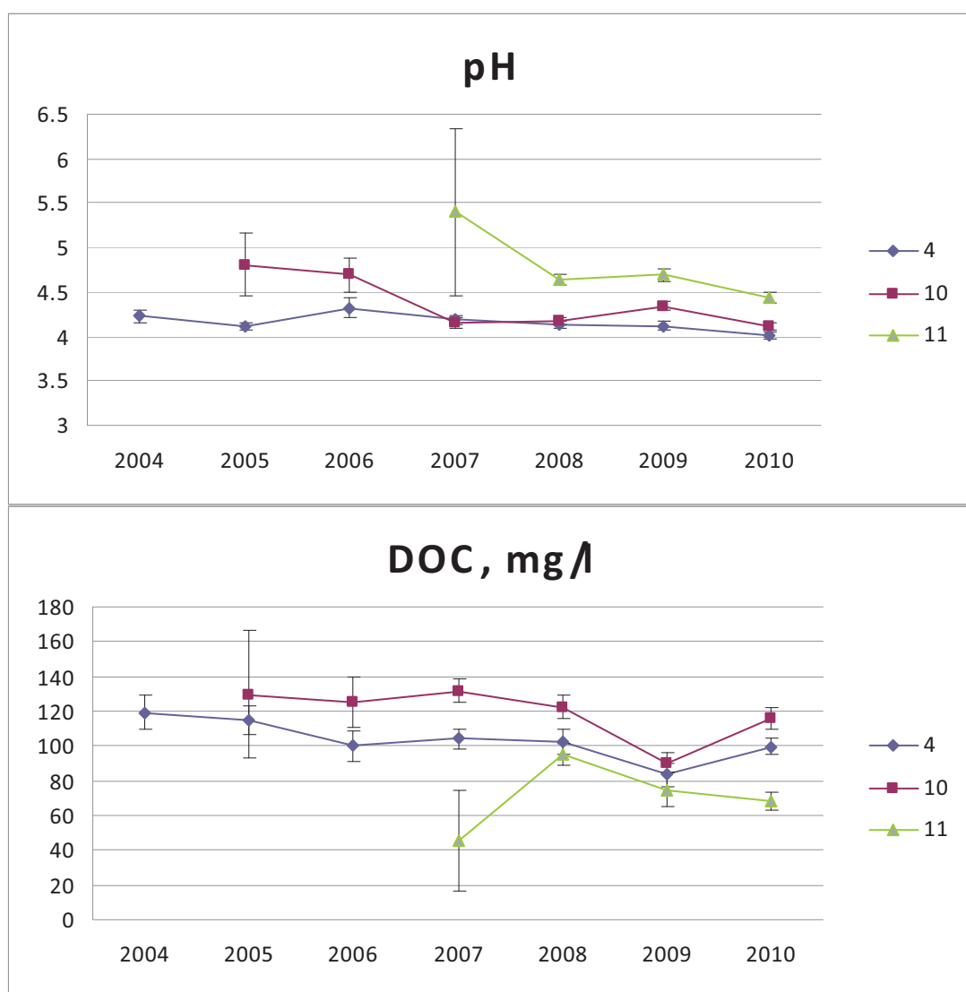
Figure 10. Annual mean pH (a) and dissolved organic carbon (DOC) (b) concentration at a depth of 5 cm on plots FIP4 (pine stand), 10 (spruce stand) and 11 (mixed stand) at Olkiluoto during the snowfree period in 2004 – 2010. The bars denote the standard error of the mean.
