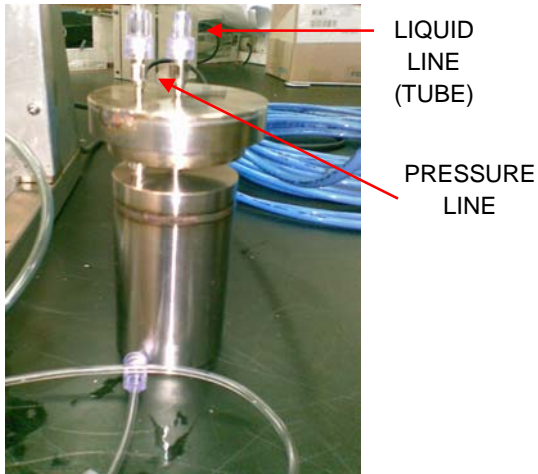
Figure 4. Tracer container
