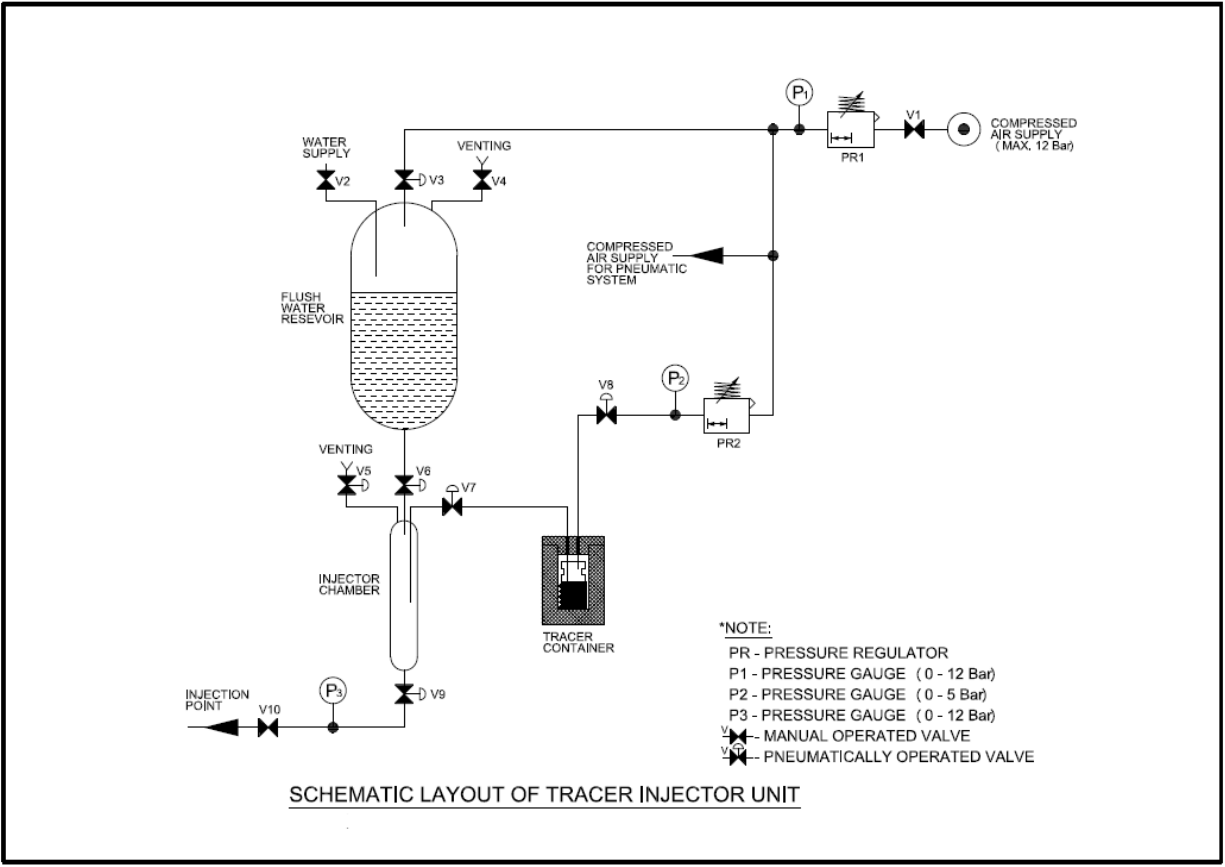
Figure 2. Schematic diagram of Radiotracer Injector-An Industrial Application (RIIA)
