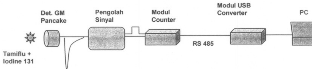
Gambar 3. Blok Diagram Deteksi Virus Flu Burung
